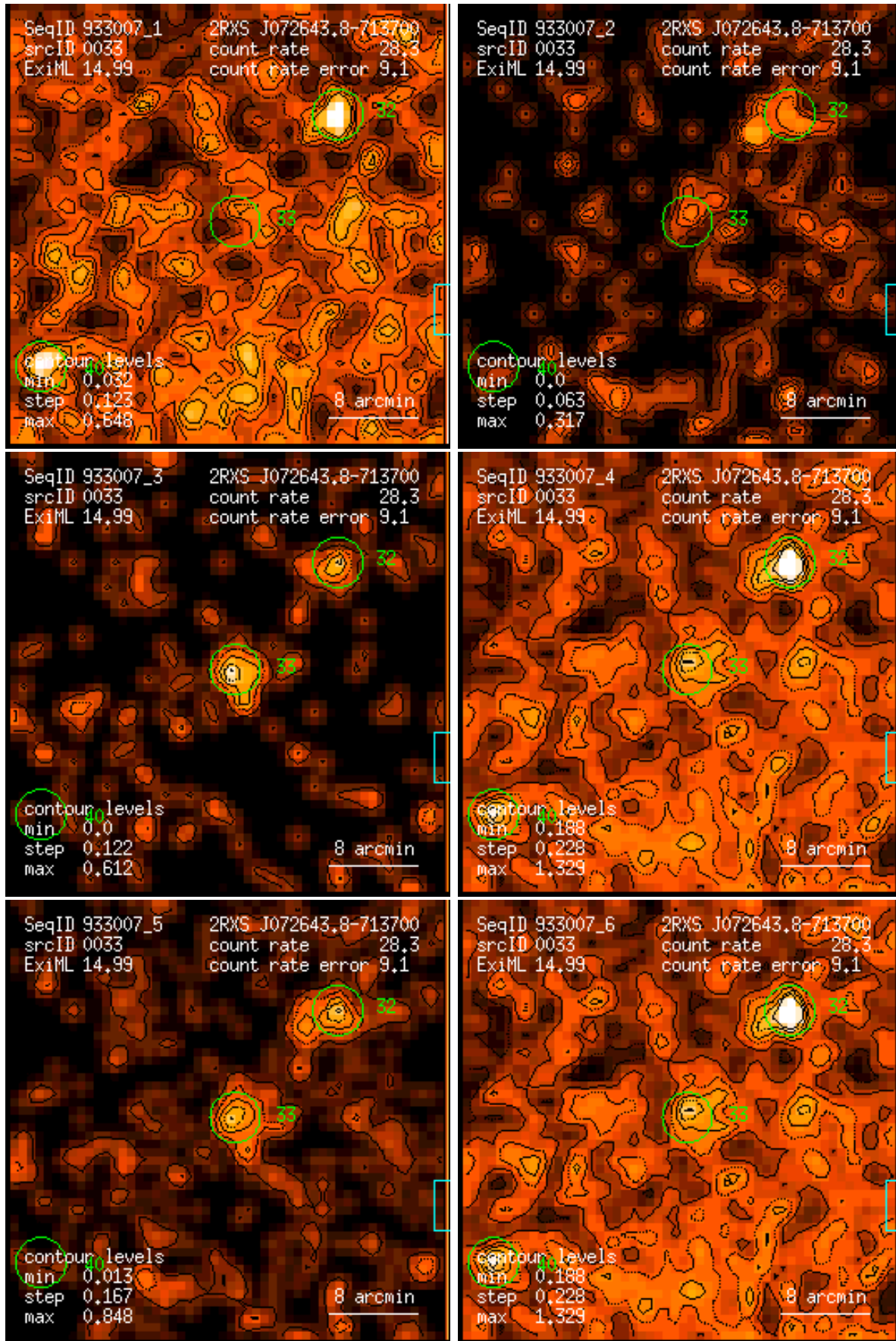
Figure 33: RASS 933007: detection 0033: band rate images, Gaussian filter: (1) PSPC channels 11 – 41, (2) 52 – 90, (3) 91 – 201, (4) 11 – 235, (5) 52 – 201, (6) 11 – 201. Broad band rates in counts/ks. Band rate contour levels in counts/ks/arcmin 2 .
