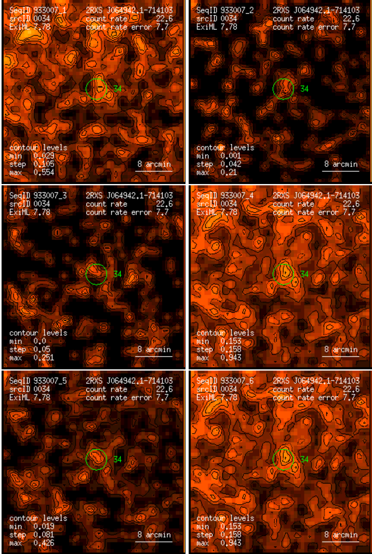
Figure 34: RASS 933007: detection 0034: band rate images, Gaussian filter: (1) PSPC channels 11 – 41, (2) 52 – 90, (3) 91 – 201, (4) 11 – 235, (5) 52 – 201, (6) 11 – 201. Broad band rates in counts/ks. Band rate contour levels in counts/ks/arcmin 2 .
