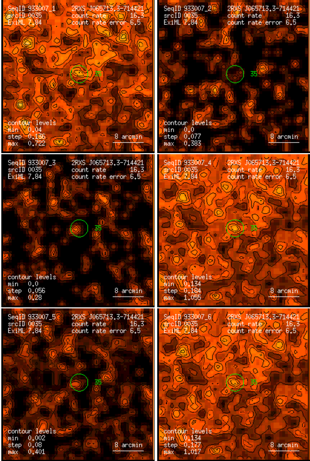
Figure 35: RASS 933007: detection 0035: band rate images, Gaussian filter: (1) PSPC channels 11 – 41, (2) 52 – 90, (3) 91 – 201, (4) 11 – 235, (5) 52 – 201, (6) 11 – 201. Broad band rates in counts/ks. Band rate contour levels in counts/ks/arcmin 2 .
