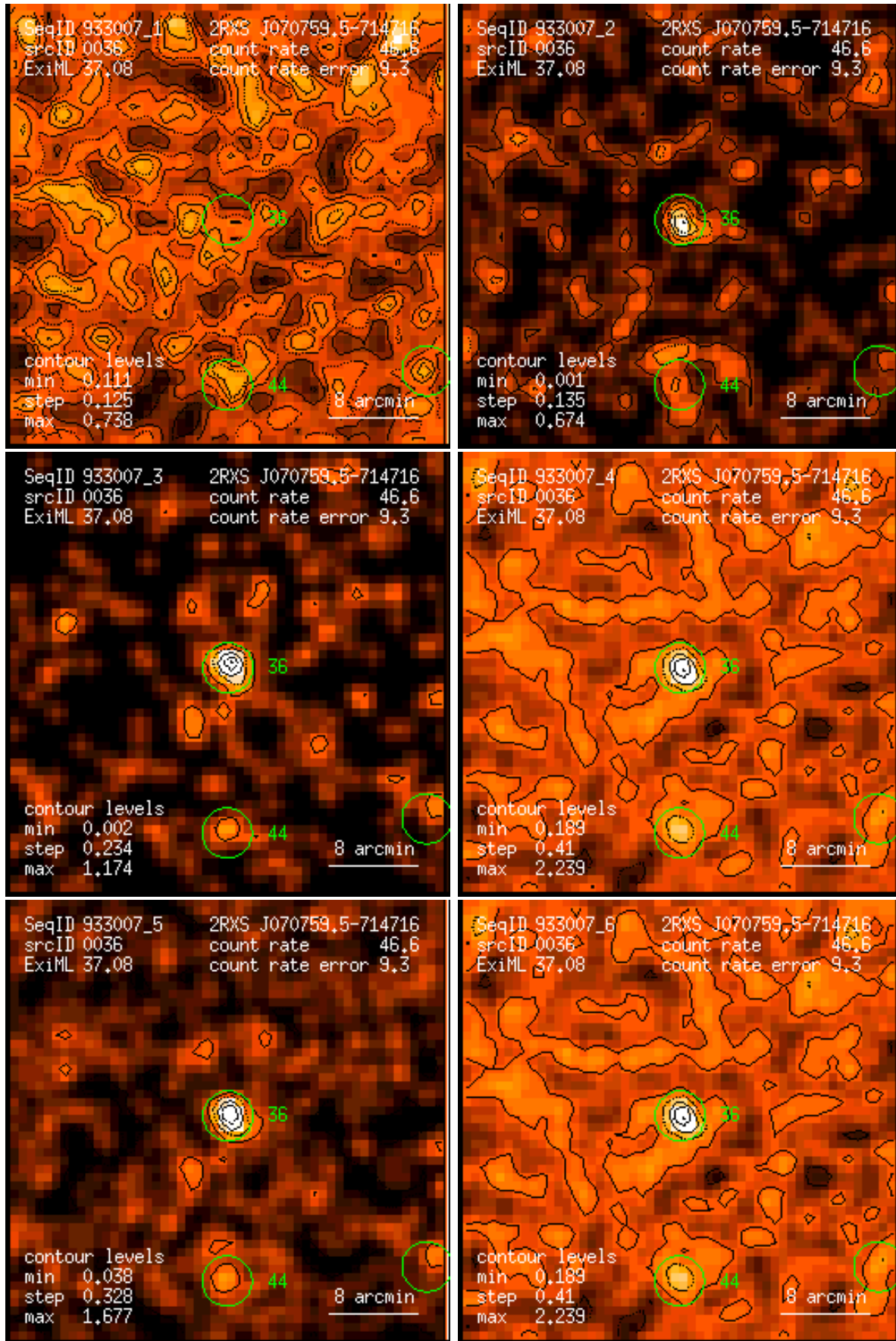
Figure 36: RASS 933007: detection 0036: band rate images, Gaussian filter: (1) PSPC channels 11 – 41, (2) 52 – 90, (3) 91 – 201, (4) 11 – 235, (5) 52 – 201, (6) 11 – 201. Broad band rates in counts/ks. Band rate contour levels in counts/ks/arcmin 2 .
