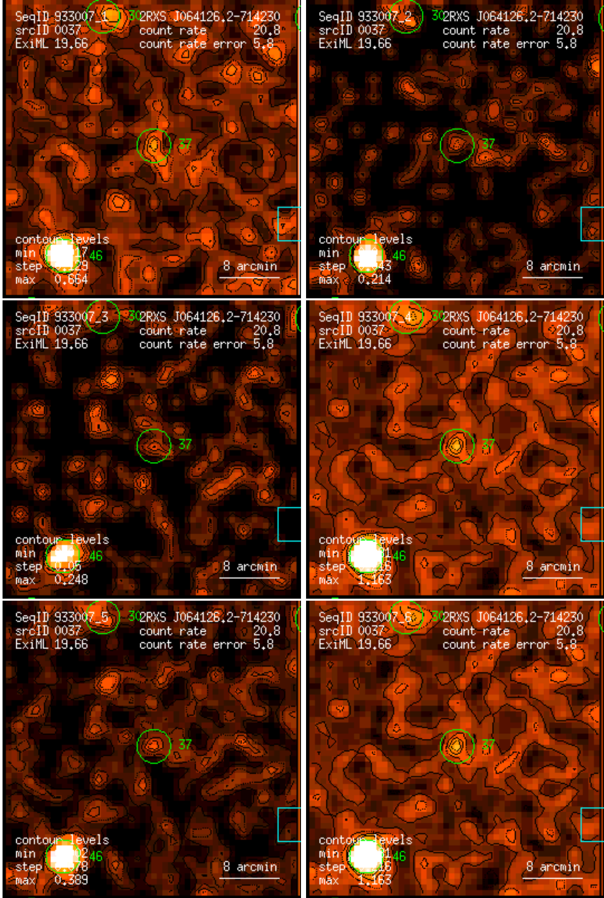
Figure 37: RASS 933007: detection 0037: band rate images, Gaussian filter: (1) PSPC channels 11 – 41, (2) 52 – 90, (3) 91 – 201, (4) 11 – 235, (5) 52 – 201, (6) 11 – 201. Broad band rates in counts/ks. Band rate contour levels in counts/ks/arcmin 2 .
