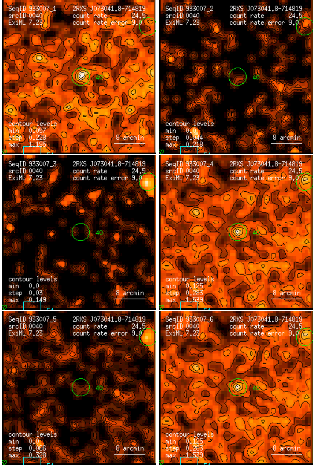
Figure 40: RASS 933007: detection 0040: band rate images, Gaussian filter: (1) PSPC channels 11 – 41, (2) 52 – 90, (3) 91 – 201, (4) 11 – 235, (5) 52 – 201, (6) 11 – 201. Broad band rates in counts/ks. Band rate contour levels in counts/ks/arcmin 2 .
