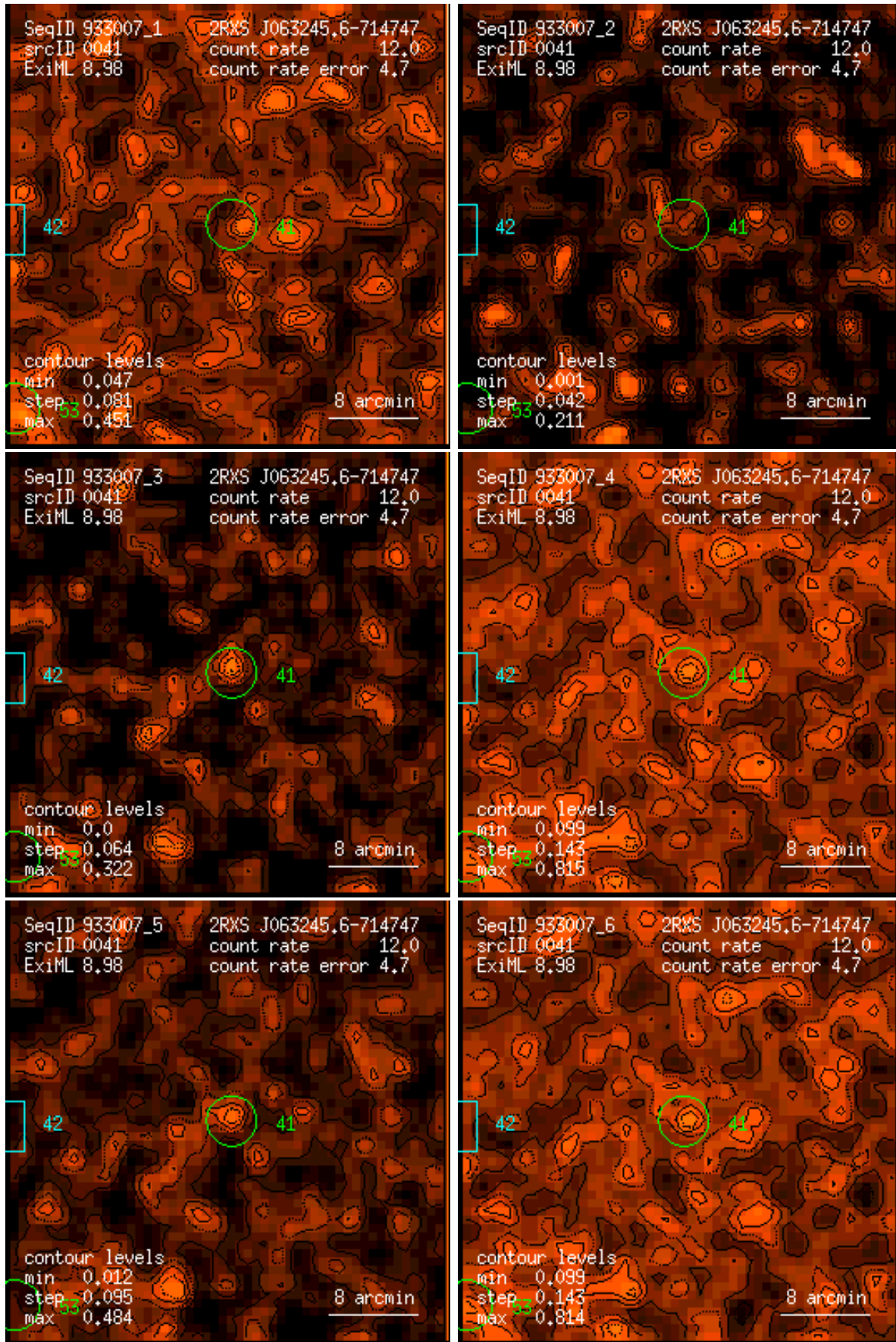
Figure 41: RASS 933007: detection 0041: band rate images, Gaussian filter: (1) PSPC channels 11 – 41, (2) 52 – 90, (3) 91 – 201, (4) 11 – 235, (5) 52 – 201, (6) 11 – 201. Broad band rates in counts/ks. Band rate contour levels in counts/ks/arcmin 2 .
