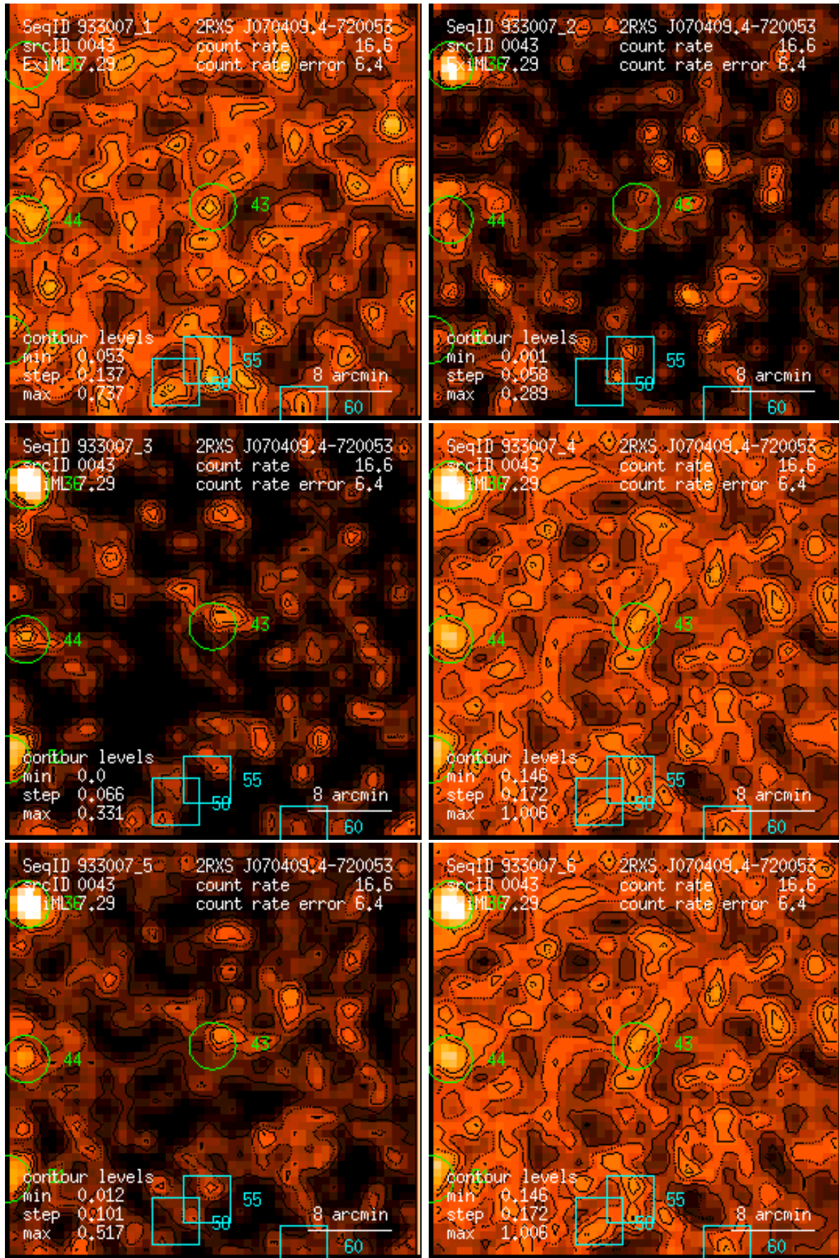
Figure 43: RASS 933007: detection 0043: band rate images, Gaussian filter: (1) PSPC channels 11 – 41, (2) 52 – 90, (3) 91 – 201, (4) 11 – 235, (5) 52 – 201, (6) 11 – 201. Broad band rates in counts/ks. Band rate contour levels in counts/ks/arcmin 2 .
