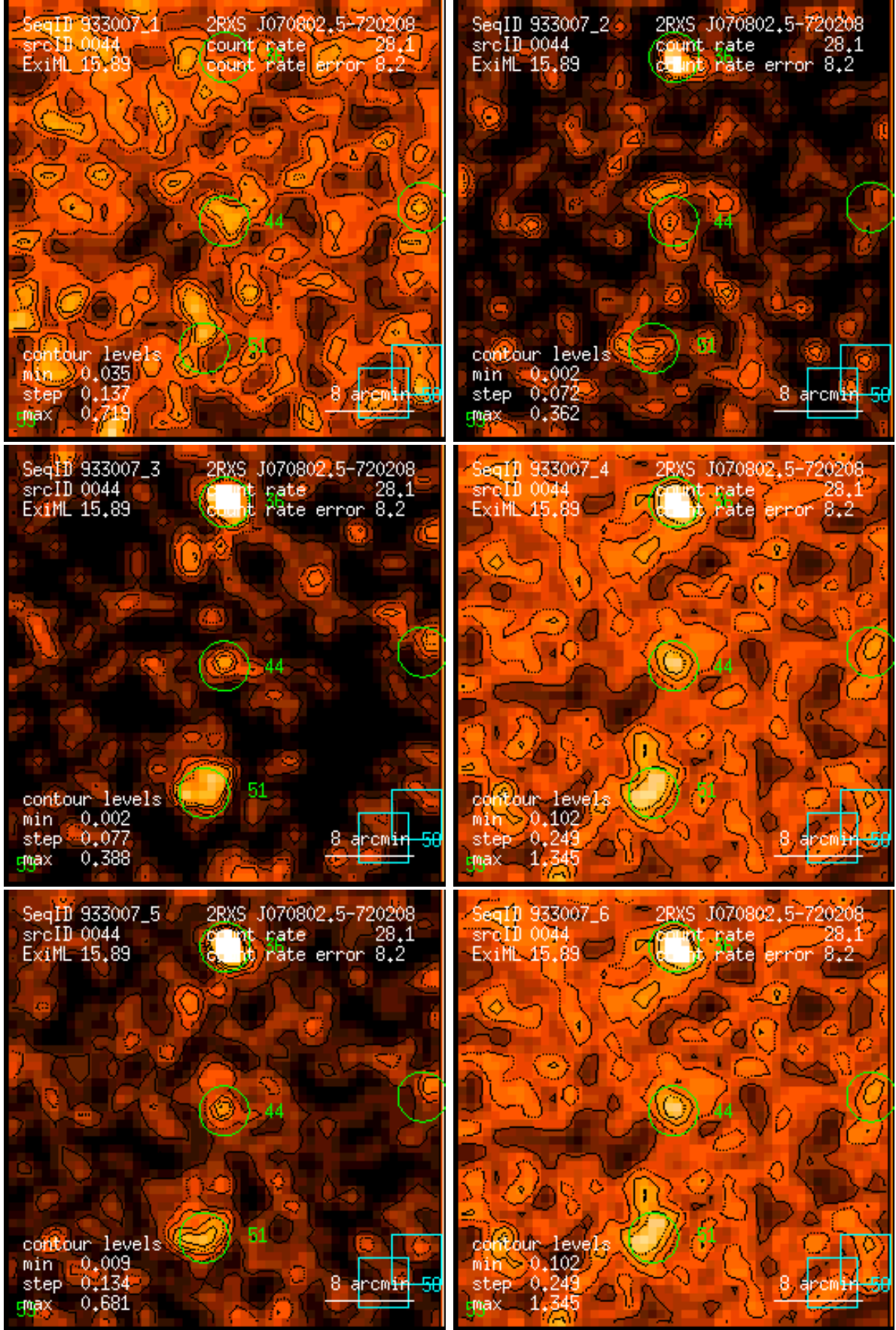
Figure 44: RASS 933007: detection 0044: band rate images, Gaussian filter: (1) PSPC channels 11 – 41, (2) 52 – 90, (3) 91 – 201, (4) 11 – 235, (5) 52 – 201, (6) 11 – 201. Broad band rates in counts/ks. Band rate contour levels in counts/ks/arcmin 2 .
