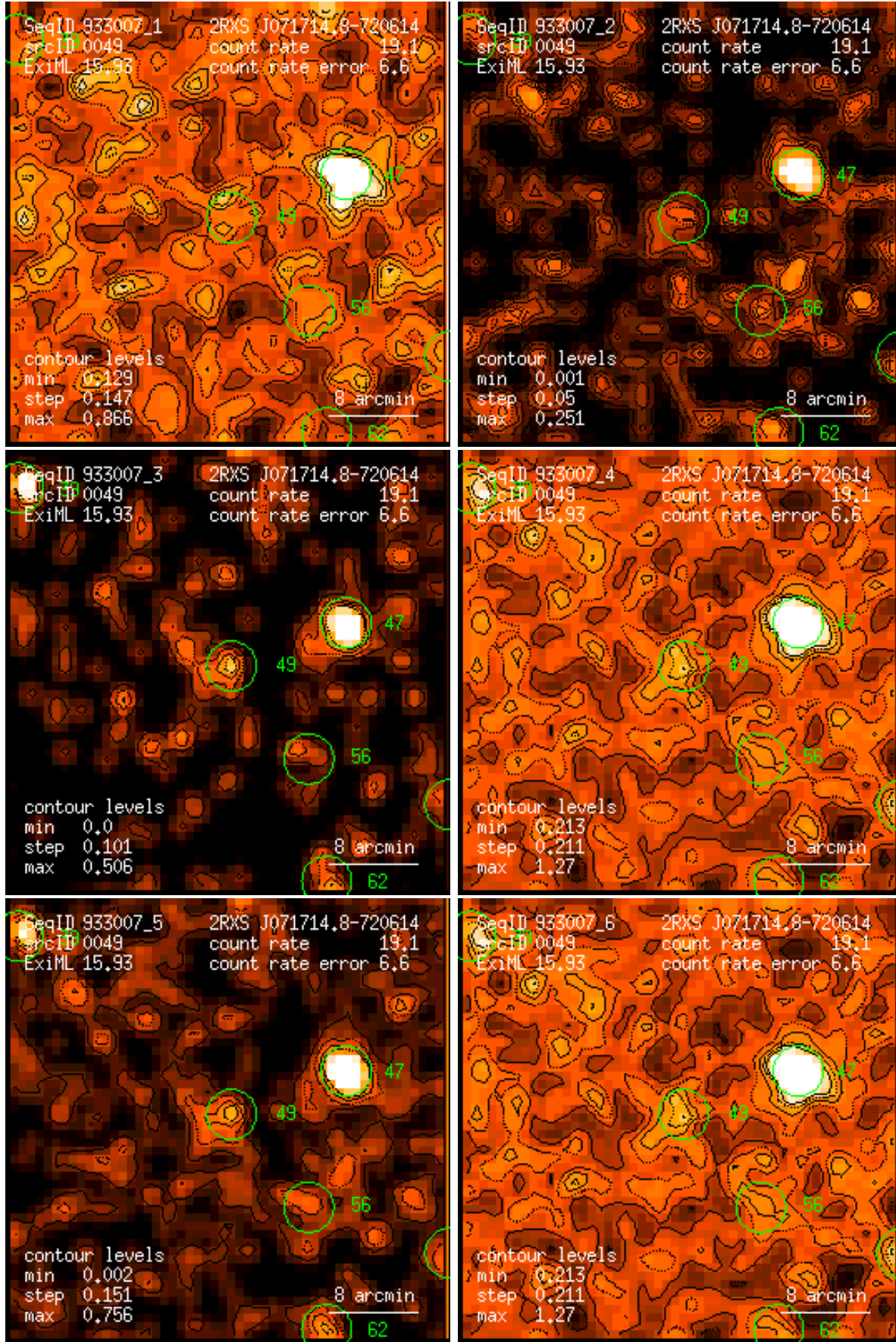
Figure 49: RASS 933007: detection 0049: band rate images, Gaussian filter: (1) PSPC channels 11 – 41, (2) 52 – 90, (3) 91 – 201, (4) 11 – 235, (5) 52 – 201, (6) 11 – 201. Broad band rates in counts/ks. Band rate contour levels in counts/ks/arcmin 2 .
