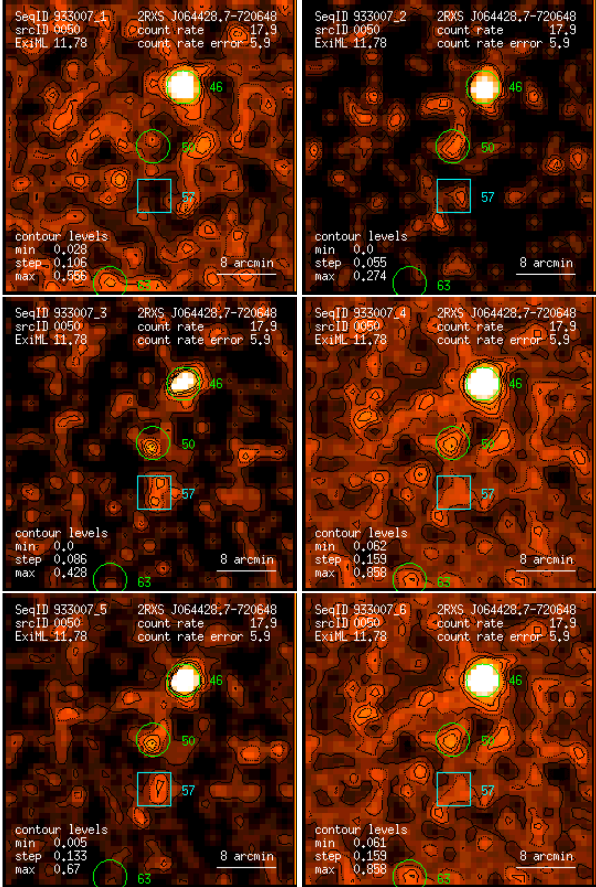
Figure 50: RASS 933007: detection 0050: band rate images, Gaussian filter: (1) PSPC channels 11 – 41, (2) 52 – 90, (3) 91 – 201, (4) 11 – 235, (5) 52 – 201, (6) 11 – 201. Broad band rates in counts/ks. Band rate contour levels in counts/ks/arcmin 2 .
