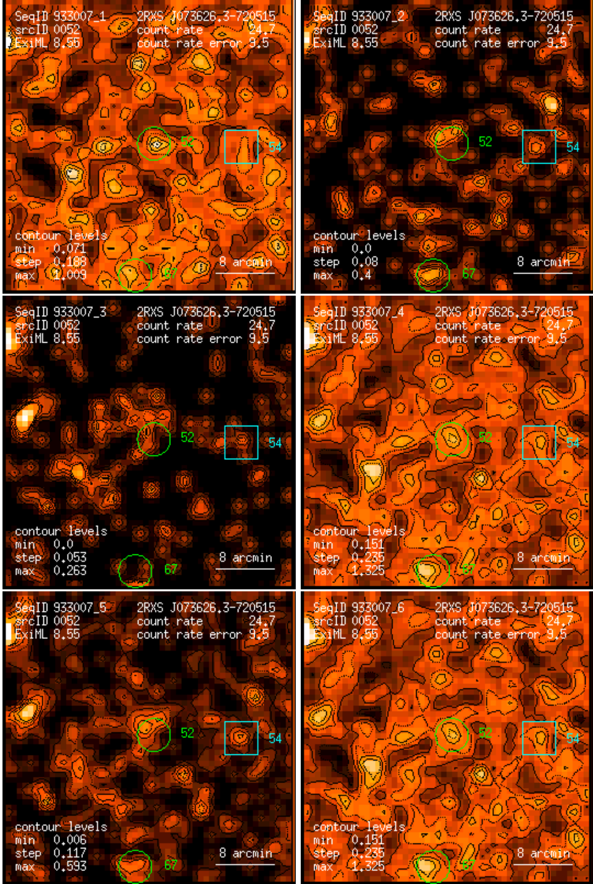
Figure 52: RASS 933007: detection 0052: band rate images, Gaussian filter: (1) PSPC channels 11 – 41, (2) 52 – 90, (3) 91 – 201, (4) 11 – 235, (5) 52 – 201, (6) 11 – 201. Broad band rates in counts/ks. Band rate contour levels in counts/ks/arcmin 2 .
