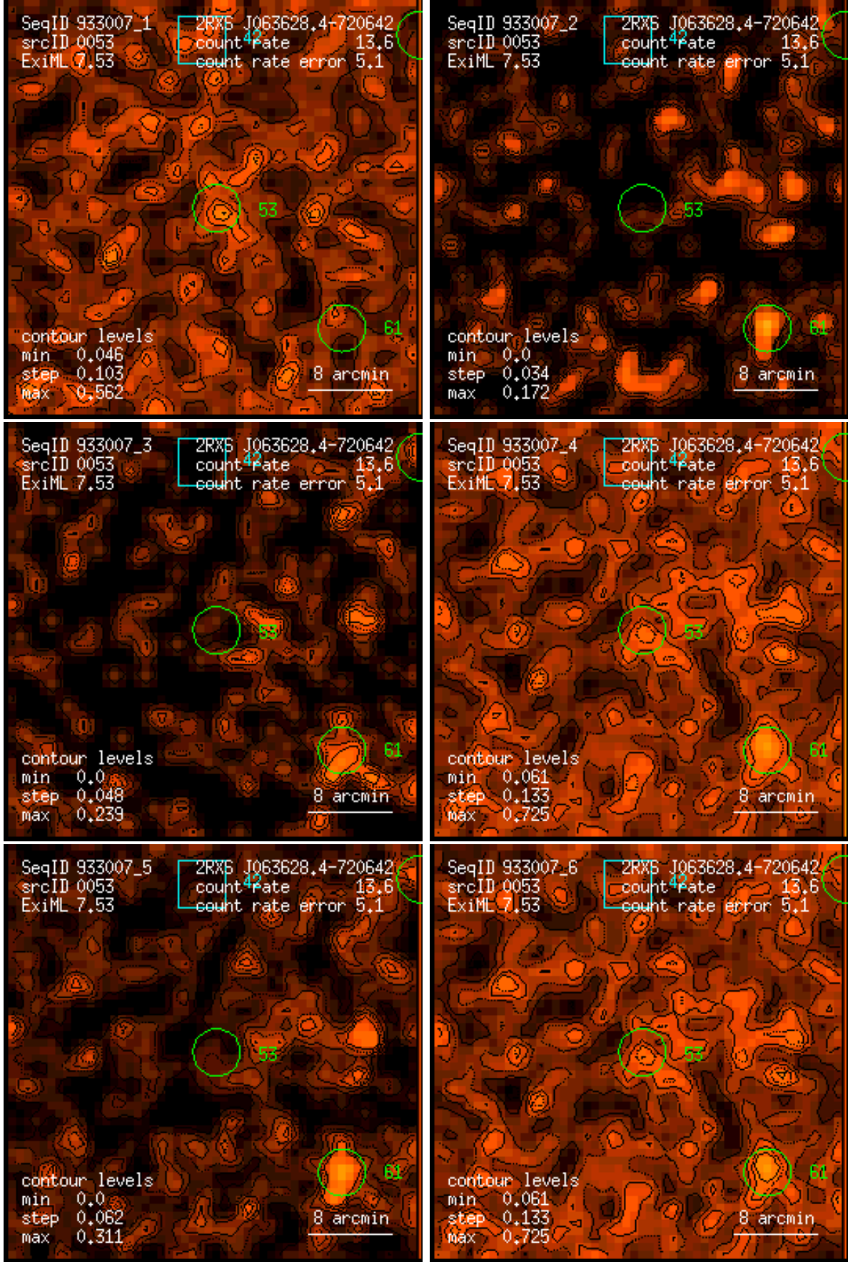
Figure 53: RASS 933007: detection 0053: band rate images, Gaussian filter: (1) PSPC channels 11 – 41, (2) 52 – 90, (3) 91 – 201, (4) 11 – 235, (5) 52 – 201, (6) 11 – 201. Broad band rates in counts/ks. Band rate contour levels in counts/ks/arcmin 2 .
