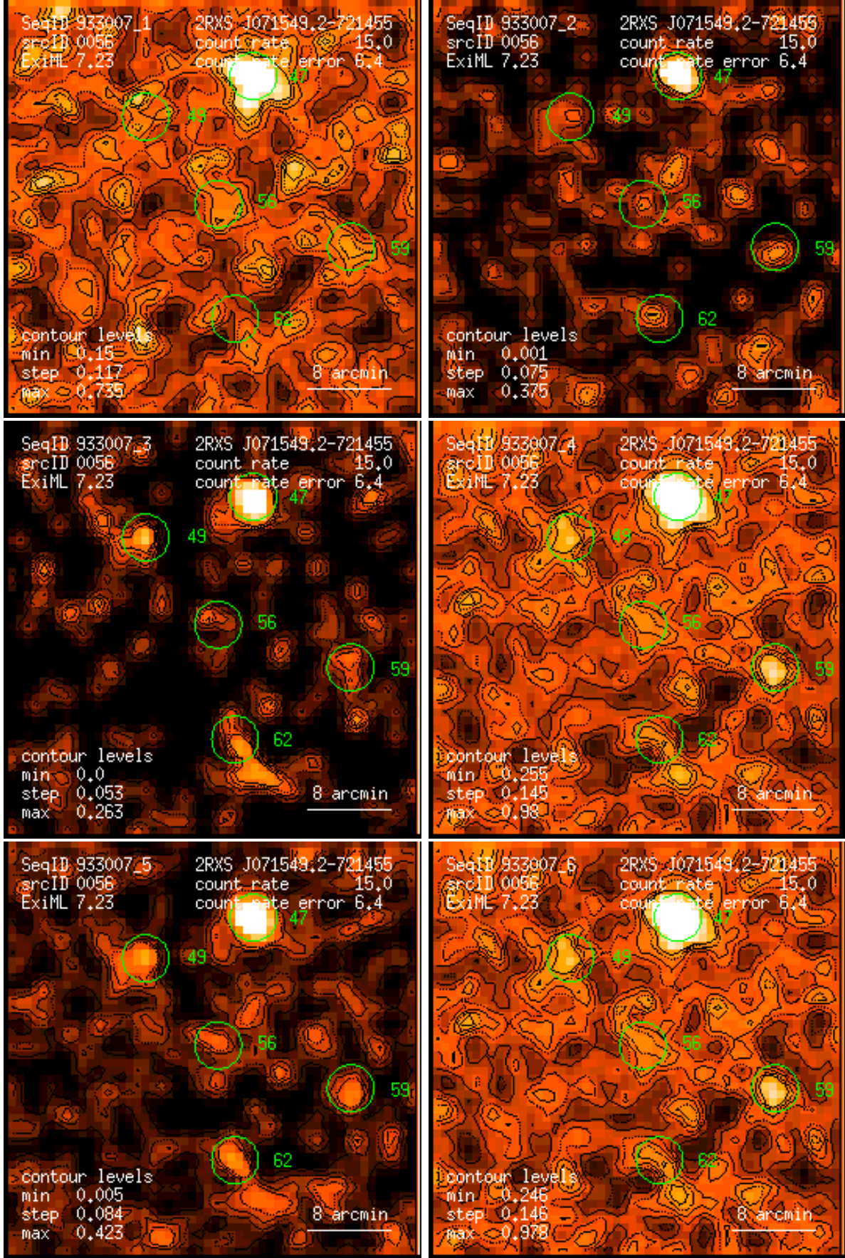
Figure 56: RASS 933007: detection 0056: band rate images, Gaussian filter: (1) PSPC channels 11 – 41, (2) 52 – 90, (3) 91 – 201, (4) 11 – 235, (5) 52 – 201, (6) 11 – 201. Broad band rates in counts/ks. Band rate contour levels in counts/ks/arcmin 2 .
