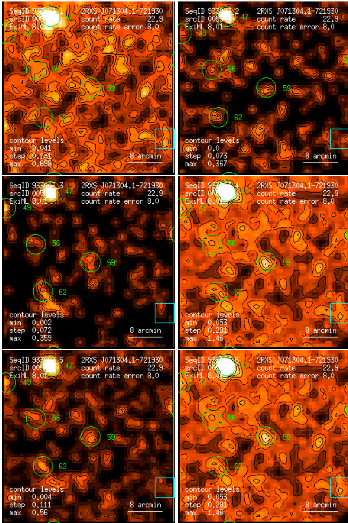
Figure 59: RASS 933007: detection 0059: band rate images, Gaussian filter: (1) PSPC channels 11 – 41, (2) 52 – 90, (3) 91 – 201, (4) 11 – 235, (5) 52 – 201, (6) 11 – 201. Broad band rates in counts/ks. Band rate contour levels in counts/ks/arcmin 2 .
