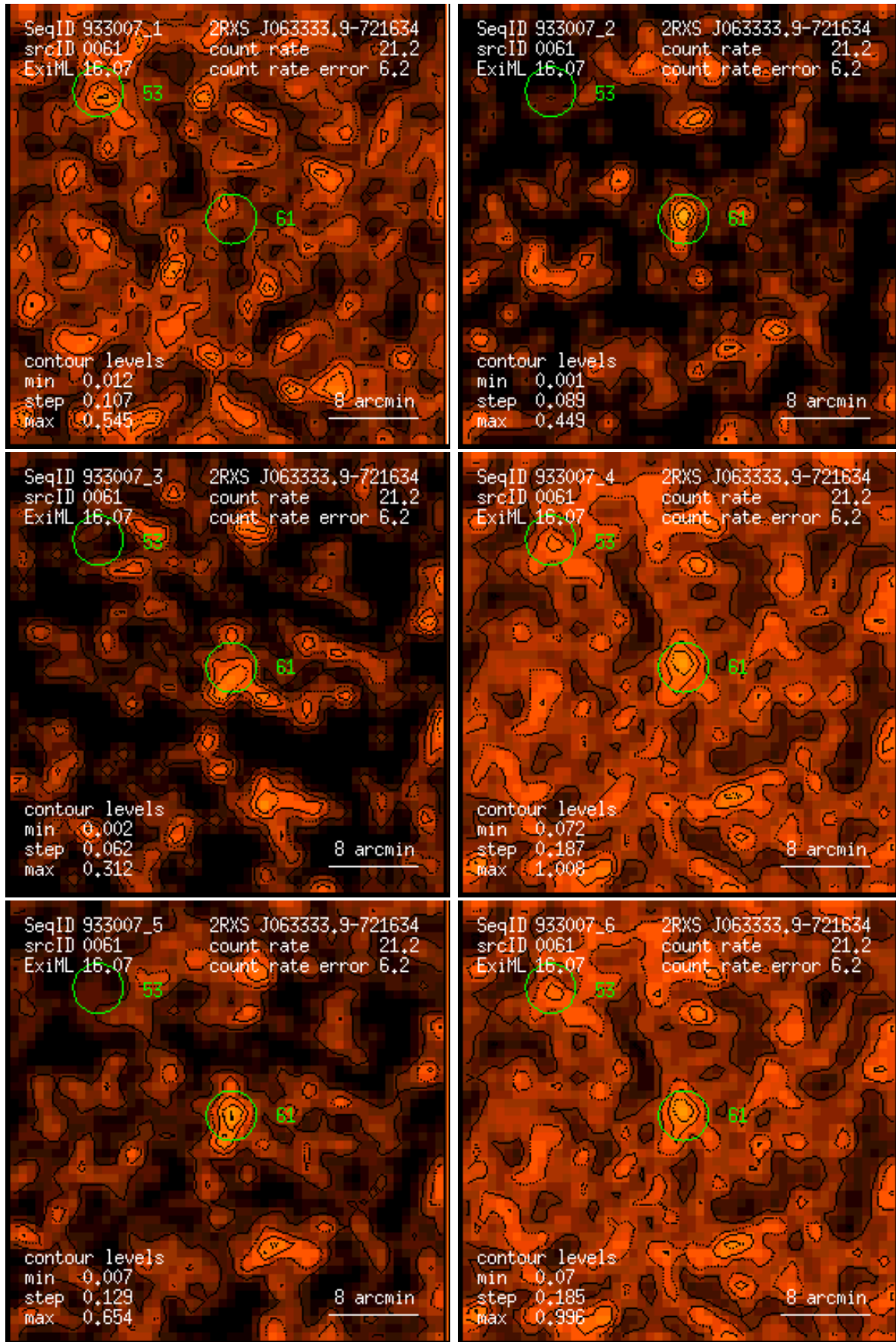
Figure 61: RASS 933007: detection 0061: band rate images, Gaussian filter: (1) PSPC channels 11 – 41, (2) 52 – 90, (3) 91 – 201, (4) 11 – 235, (5) 52 – 201, (6) 11 – 201. Broad band rates in counts/ks. Band rate contour levels in counts/ks/arcmin 2 .
