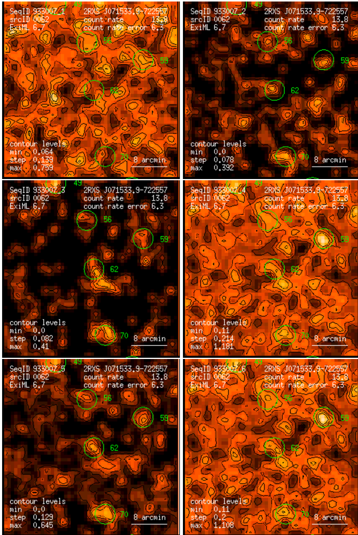
Figure 62: RASS 933007: detection 0062: band rate images, Gaussian filter: (1) PSPC channels 11 – 41, (2) 52 – 90, (3) 91 – 201, (4) 11 – 235, (5) 52 – 201, (6) 11 – 201. Broad band rates in counts/ks. Band rate contour levels in counts/ks/arcmin 2 .
