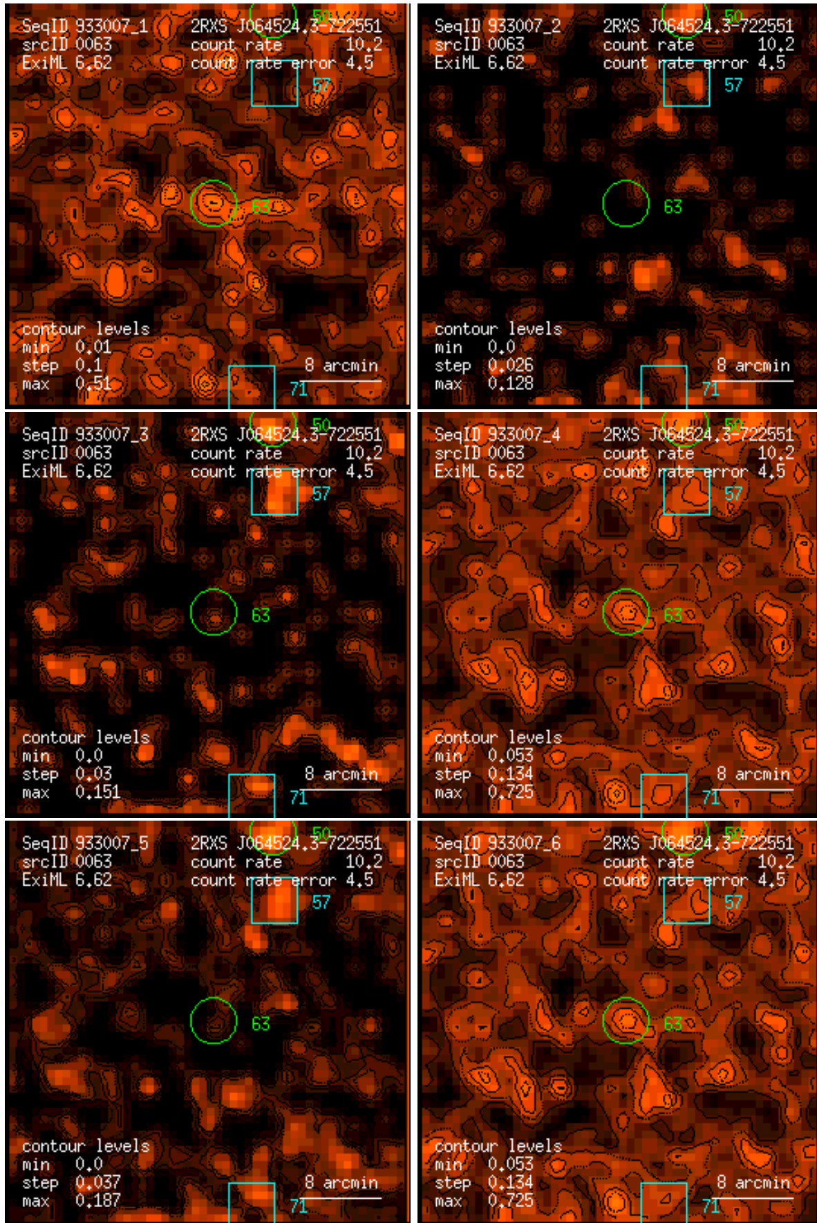
Figure 63: RASS 933007: detection 0063: band rate images, Gaussian filter: (1) PSPC channels 11 – 41, (2) 52 – 90, (3) 91 – 201, (4) 11 – 235, (5) 52 – 201, (6) 11 – 201. Broad band rates in counts/ks. Band rate contour levels in counts/ks/arcmin 2 .
