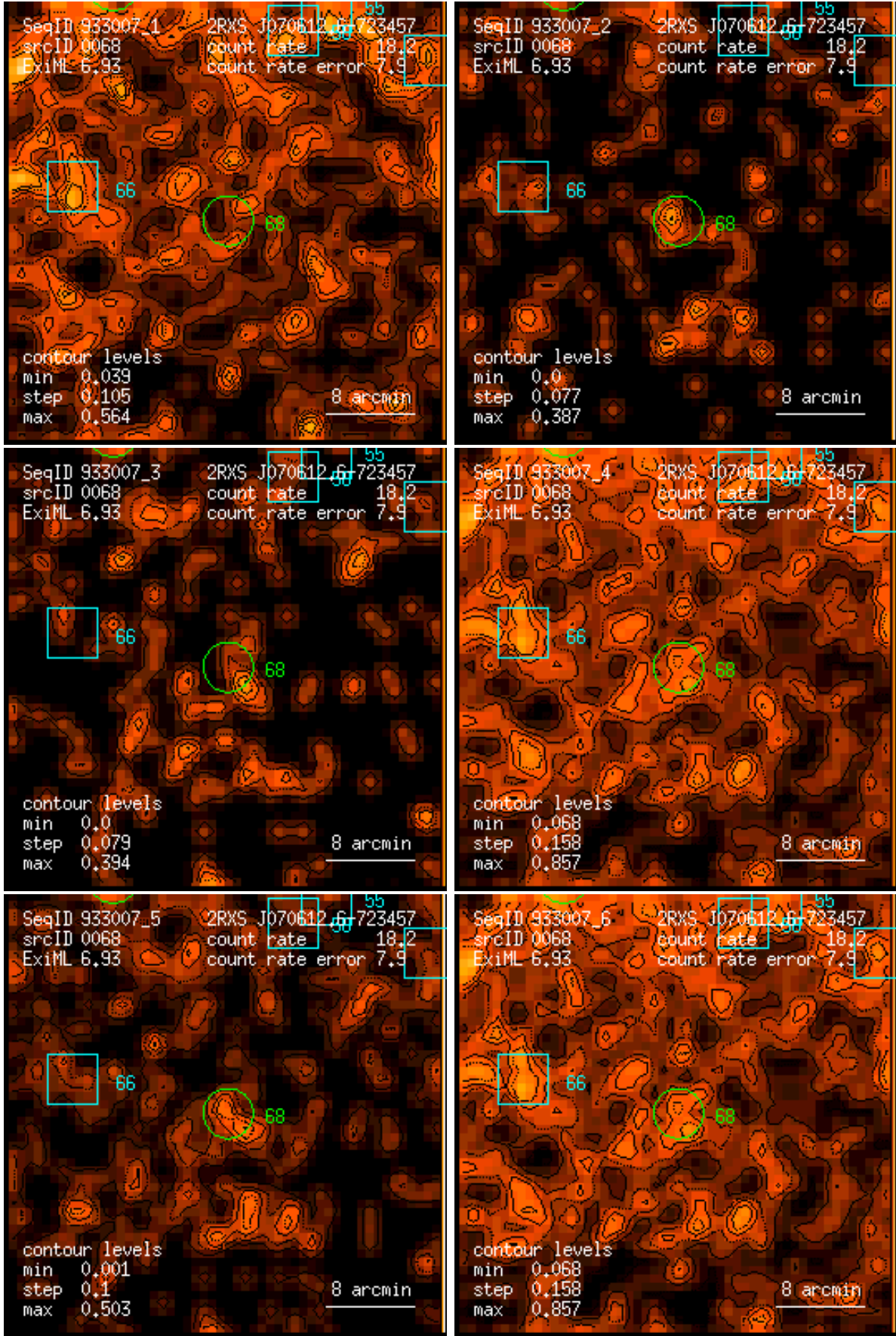
Figure 68: RASS 933007: detection 0068: band rate images, Gaussian filter: (1) PSPC channels 11 – 41, (2) 52 – 90, (3) 91 – 201, (4) 11 – 235, (5) 52 – 201, (6) 11 – 201. Broad band rates in counts/ks. Band rate contour levels in counts/ks/arcmin 2 .
