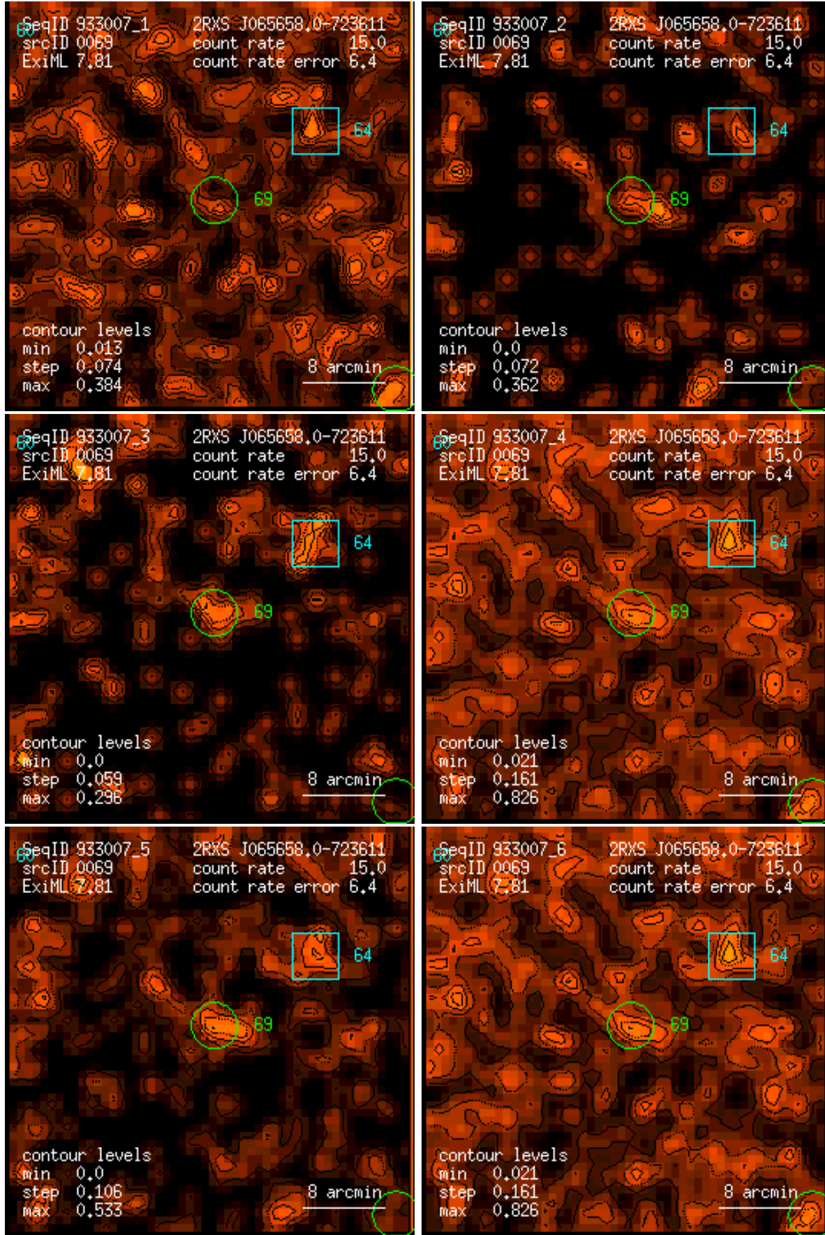
Figure 69: RASS 933007: detection 0069: band rate images, Gaussian filter: (1) PSPC channels 11 – 41, (2) 52 – 90, (3) 91 – 201, (4) 11 – 235, (5) 52 – 201, (6) 11 – 201. Broad band rates in counts/ks. Band rate contour levels in counts/ks/arcmin 2 .
