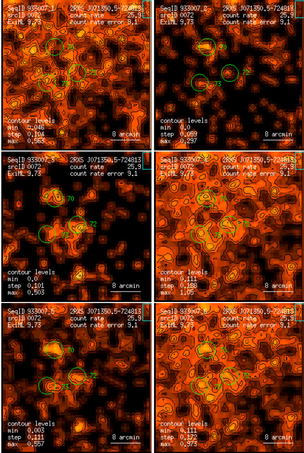
Figure 72: RASS 933007: detection 0072: band rate images, Gaussian filter: (1) PSPC channels 11 – 41, (2) 52 – 90, (3) 91 – 201, (4) 11 – 235, (5) 52 – 201, (6) 11 – 201. Broad band rates in counts/ks. Band rate contour levels in counts/ks/arcmin 2 .
