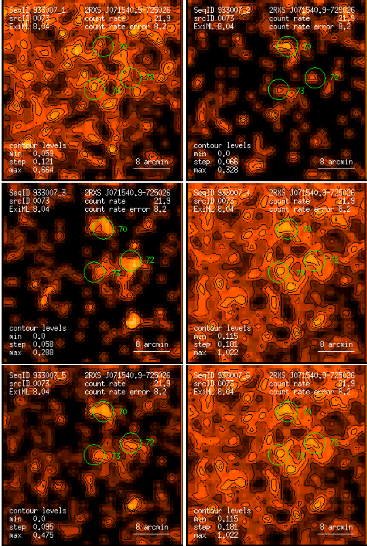
Figure 73: RASS 933007: detection 0073: band rate images, Gaussian filter: (1) PSPC channels 11 – 41, (2) 52 – 90, (3) 91 – 201, (4) 11 – 235, (5) 52 – 201, (6) 11 – 201. Broad band rates in counts/ks. Band rate contour levels in counts/ks/arcmin 2 .
