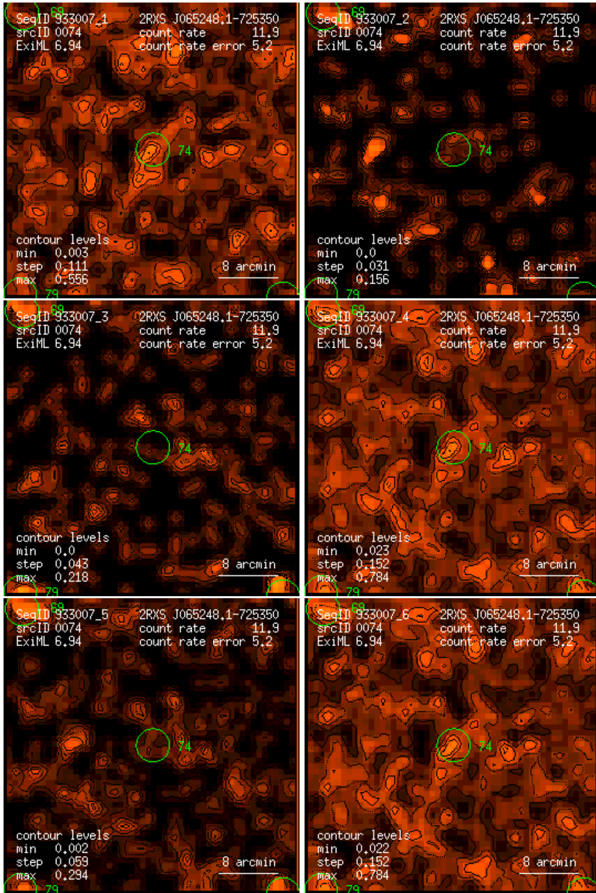
Figure 74: RASS 933007: detection 0074: band rate images, Gaussian filter: (1) PSPC channels 11 – 41, (2) 52 – 90, (3) 91 – 201, (4) 11 – 235, (5) 52 – 201, (6) 11 – 201. Broad band rates in counts/ks. Band rate contour levels in counts/ks/arcmin 2 .
