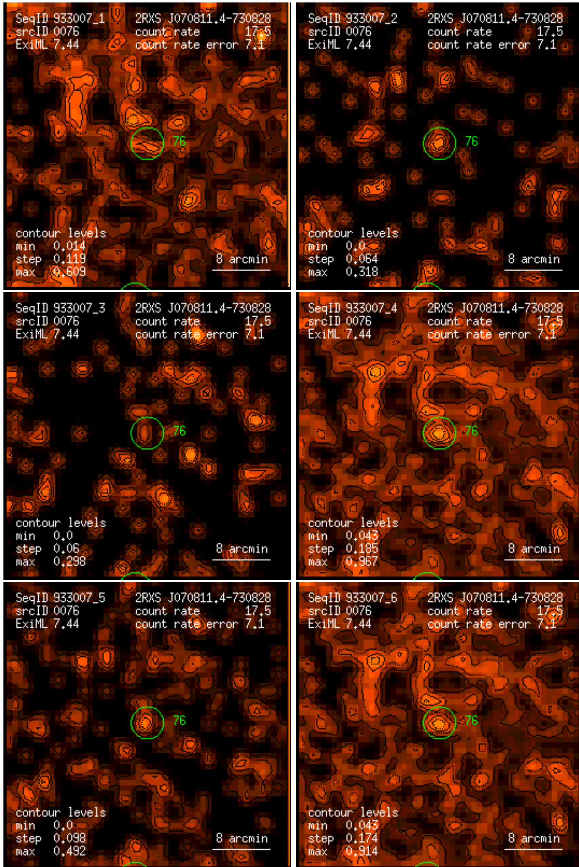
Figure 76: RASS 933007: detection 0076: band rate images, Gaussian filter: (1) PSPC channels 11 – 41, (2) 52 – 90, (3) 91 – 201, (4) 11 – 235, (5) 52 – 201, (6) 11 – 201. Broad band rates in counts/ks. Band rate contour levels in counts/ks/arcmin 2 .
