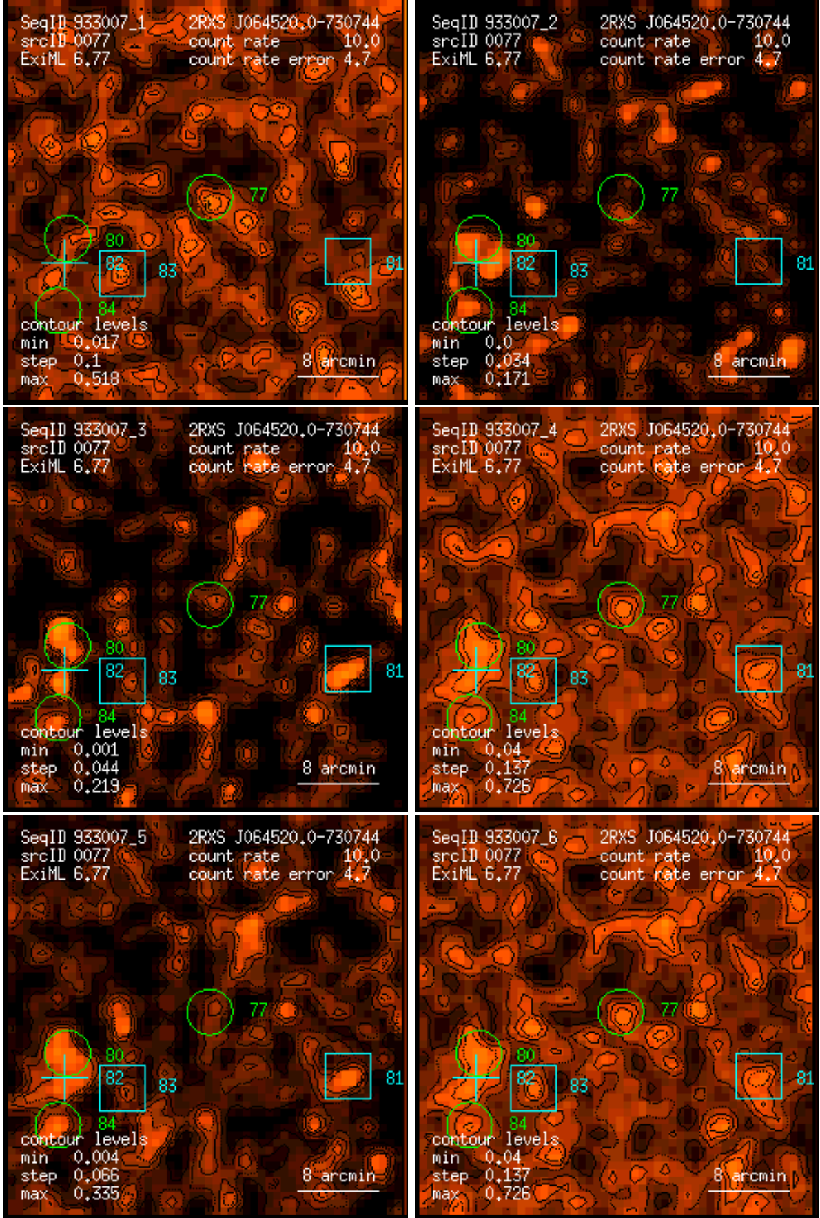
Figure 77: RASS 933007: detection 0077: band rate images, Gaussian filter: (1) PSPC channels 11 – 41, (2) 52 – 90, (3) 91 – 201, (4) 11 – 235, (5) 52 – 201, (6) 11 – 201. Broad band rates in counts/ks. Band rate contour levels in counts/ks/arcmin 2 .
