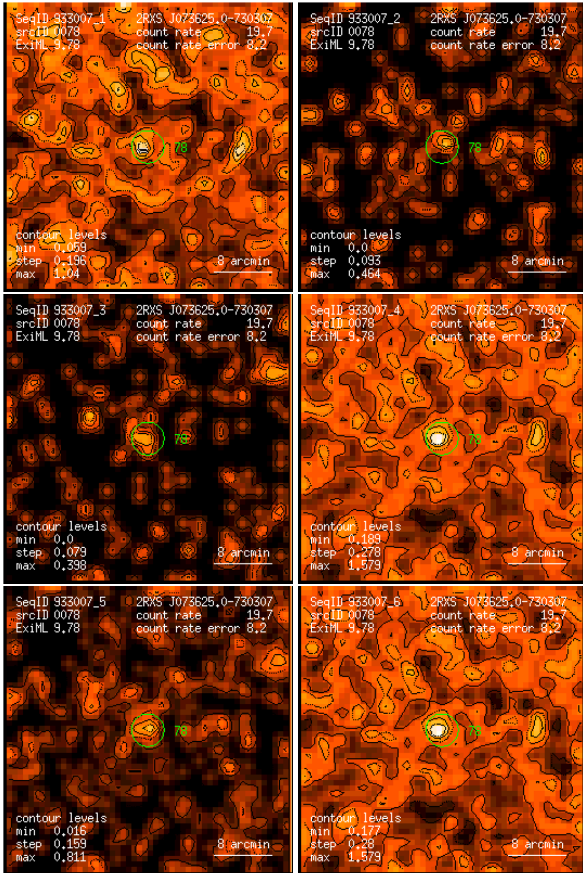
Figure 78: RASS 933007: detection 0078: band rate images, Gaussian filter: (1) PSPC channels 11 – 41, (2) 52 – 90, (3) 91 – 201, (4) 11 – 235, (5) 52 – 201, (6) 11 – 201. Broad band rates in counts/ks. Band rate contour levels in counts/ks/arcmin 2 .
