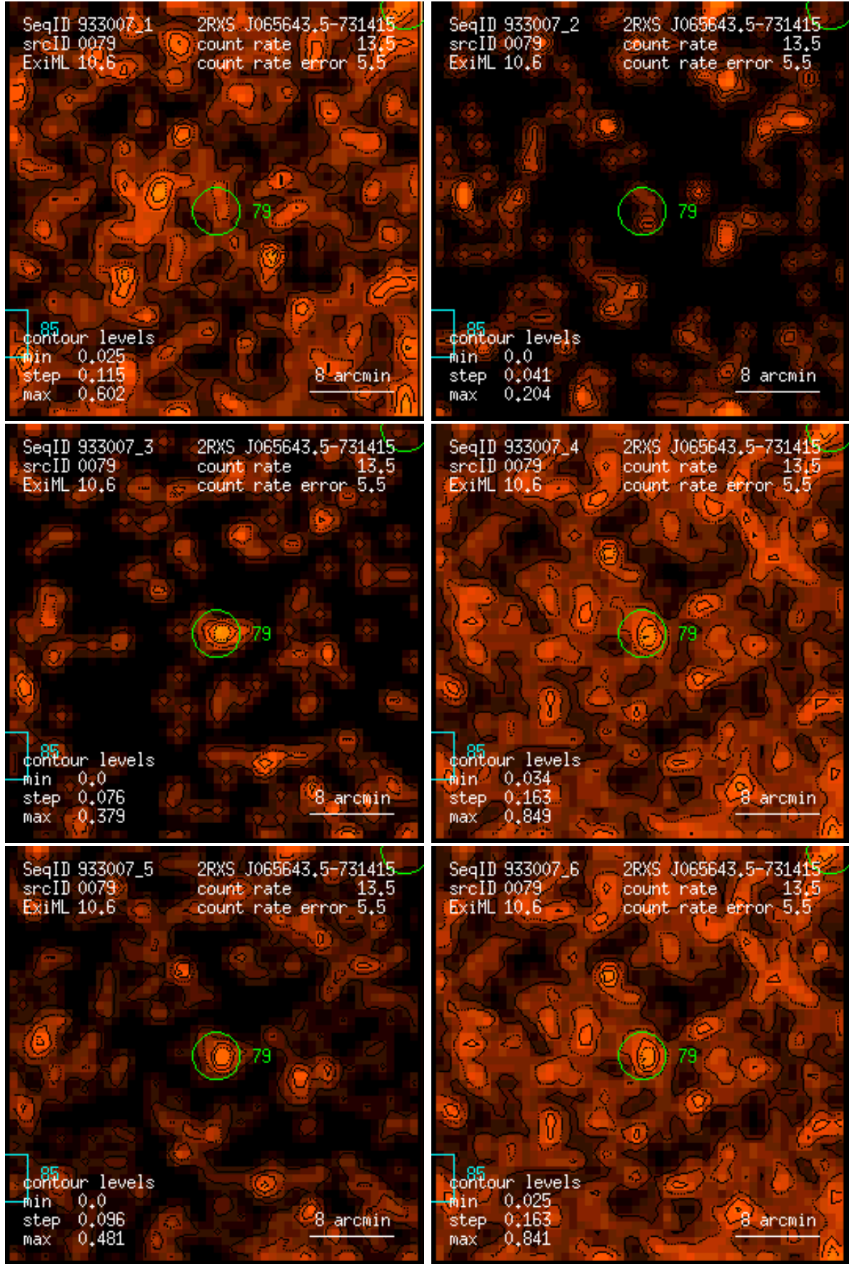
Figure 79: RASS 933007: detection 0079: band rate images, Gaussian filter: (1) PSPC channels 11 – 41, (2) 52 – 90, (3) 91 – 201, (4) 11 – 235, (5) 52 – 201, (6) 11 – 201. Broad band rates in counts/ks. Band rate contour levels in counts/ks/arcmin 2 .
