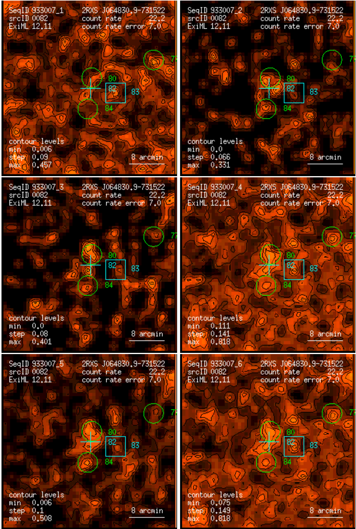
Figure 82: RASS 933007: detection 0082: band rate images, Gaussian filter: (1) PSPC channels 11 – 41, (2) 52 – 90, (3) 91 – 201, (4) 11 – 235, (5) 52 – 201, (6) 11 – 201. Broad band rates in counts/ks. Band rate contour levels in counts/ks/arcmin 2 .
