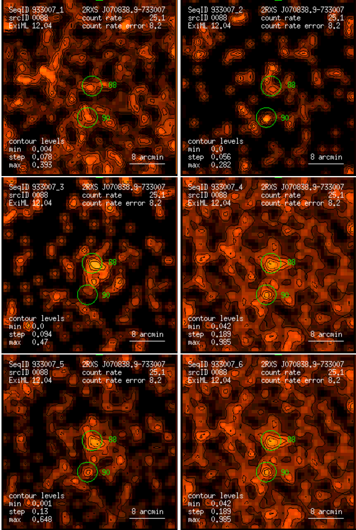
Figure 88: RASS 933007: detection 0088: band rate images, Gaussian filter: (1) PSPC channels 11 – 41, (2) 52 – 90, (3) 91 – 201, (4) 11 – 235, (5) 52 – 201, (6) 11 – 201. Broad band rates in counts/ks. Band rate contour levels in counts/ks/arcmin 2 .
