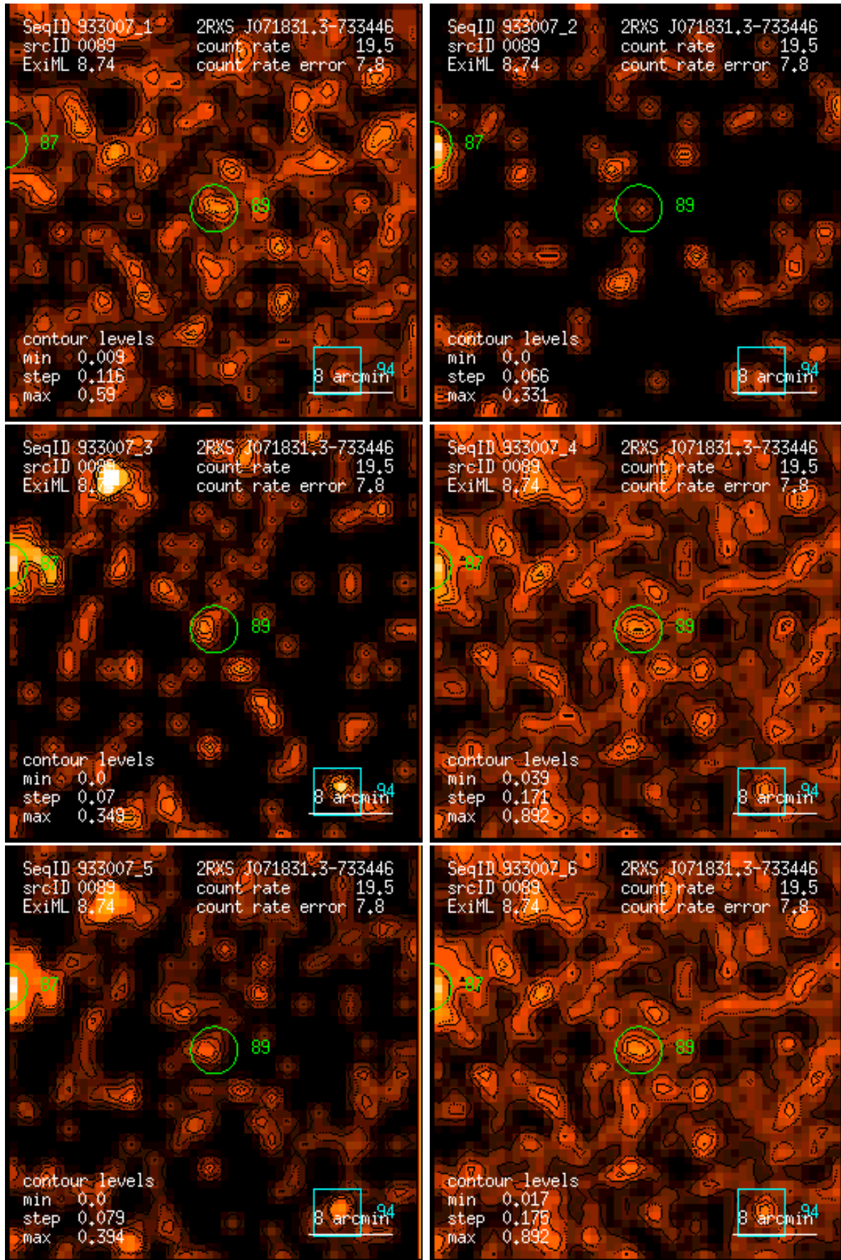
Figure 89: RASS 933007: detection 0089: band rate images, Gaussian filter: (1) PSPC channels 11 – 41, (2) 52 – 90, (3) 91 – 201, (4) 11 – 235, (5) 52 – 201, (6) 11 – 201. Broad band rates in counts/ks. Band rate contour levels in counts/ks/arcmin 2 .
