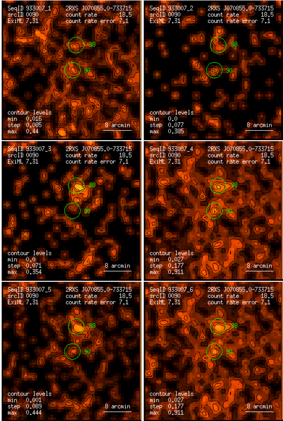
Figure 90: RASS 933007: detection 0090: band rate images, Gaussian filter: (1) PSPC channels 11 – 41, (2) 52 – 90, (3) 91 – 201, (4) 11 – 235, (5) 52 – 201, (6) 11 – 201. Broad band rates in counts/ks. Band rate contour levels in counts/ks/arcmin 2 .
