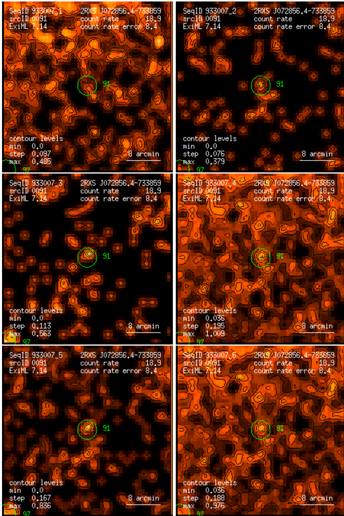
Figure 91: RASS 933007: detection 0091: band rate images, Gaussian filter: (1) PSPC channels 11 – 41, (2) 52 – 90, (3) 91 – 201, (4) 11 – 235, (5) 52 – 201, (6) 11 – 201. Broad band rates in counts/ks. Band rate contour levels in counts/ks/arcmin 2 .
