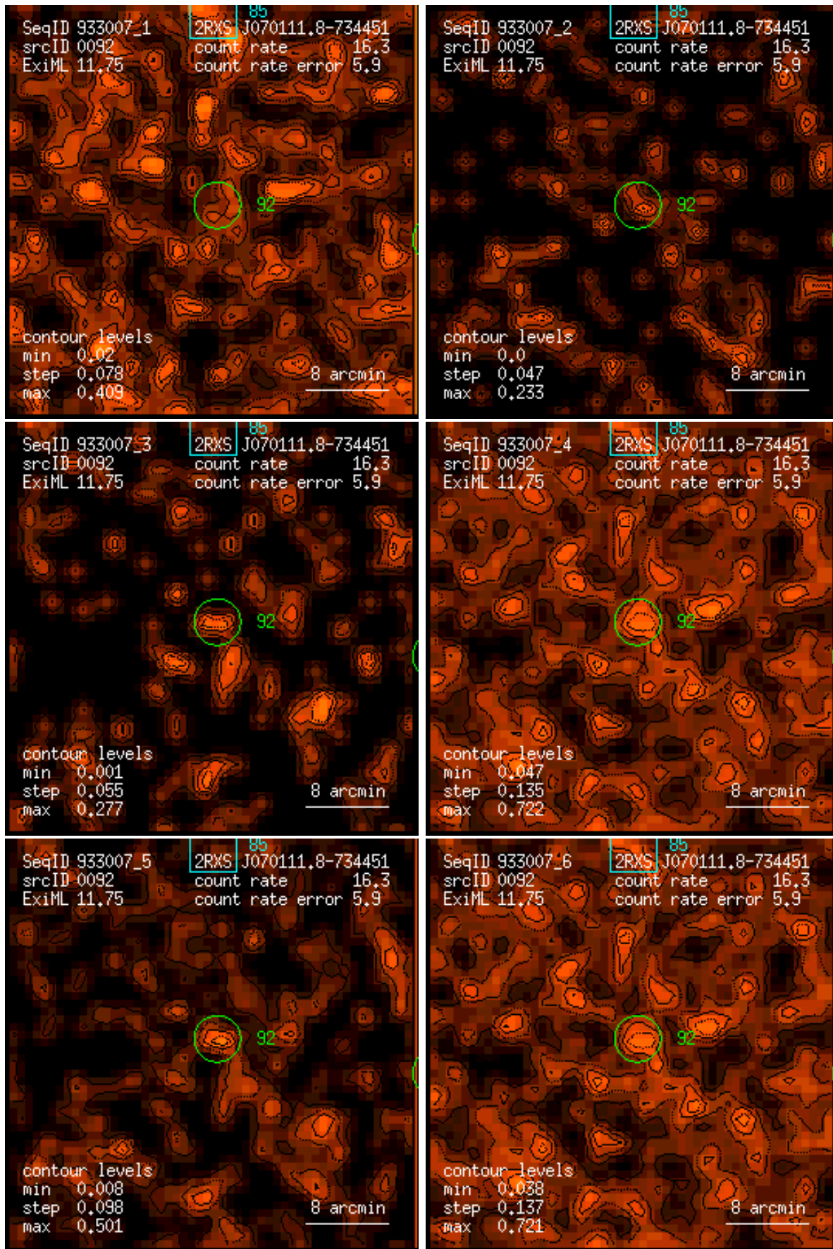
Figure 92: RASS 933007: detection 0092: band rate images, Gaussian filter: (1) PSPC channels 11 – 41, (2) 52 – 90, (3) 91 – 201, (4) 11 – 235, (5) 52 – 201, (6) 11 – 201. Broad band rates in counts/ks. Band rate contour levels in counts/ks/arcmin 2 .
