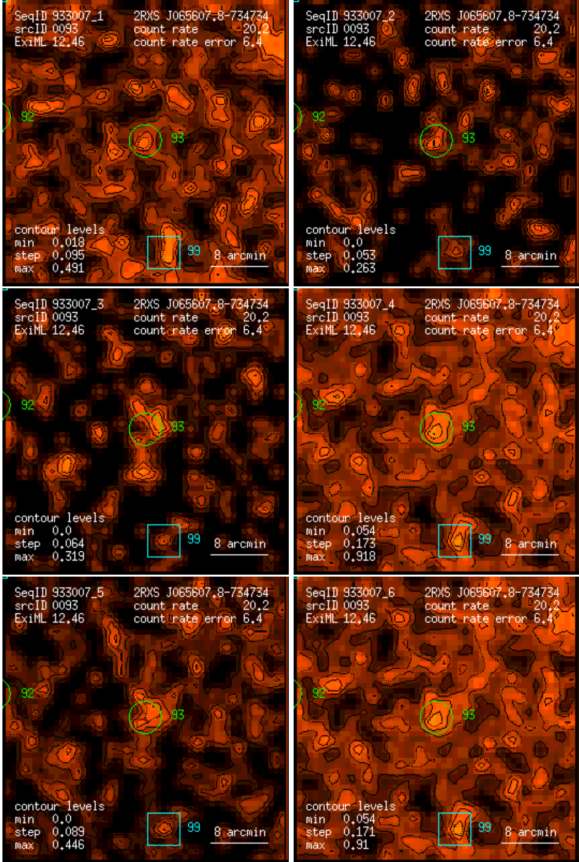
Figure 93: RASS 933007: detection 0093: band rate images, Gaussian filter: (1) PSPC channels 11 – 41, (2) 52 – 90, (3) 91 – 201, (4) 11 – 235, (5) 52 – 201, (6) 11 – 201. Broad band rates in counts/ks. Band rate contour levels in counts/ks/arcmin 2 .
