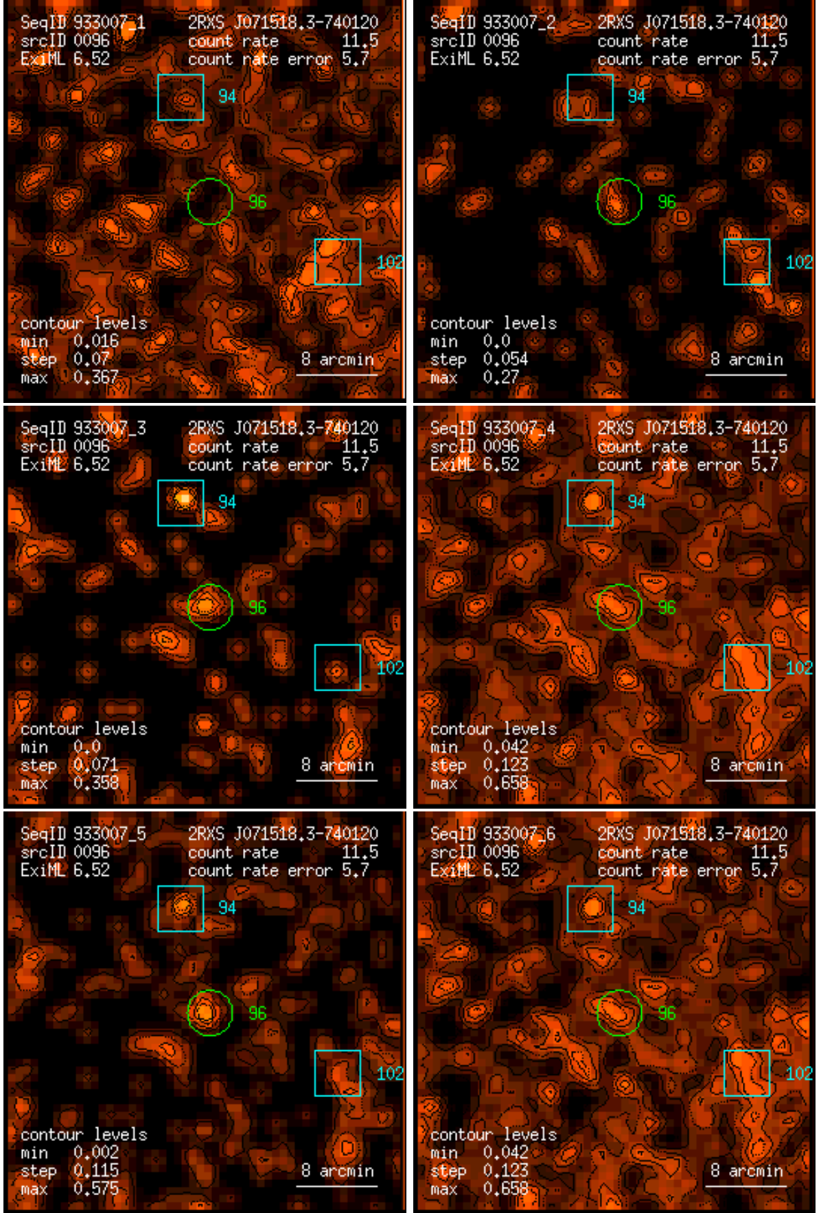
Figure 96: RASS 933007: detection 0096: band rate images, Gaussian filter: (1) PSPC channels 11 – 41, (2) 52 – 90, (3) 91 – 201, (4) 11 – 235, (5) 52 – 201, (6) 11 – 201. Broad band rates in counts/ks. Band rate contour levels in counts/ks/arcmin 2 .
