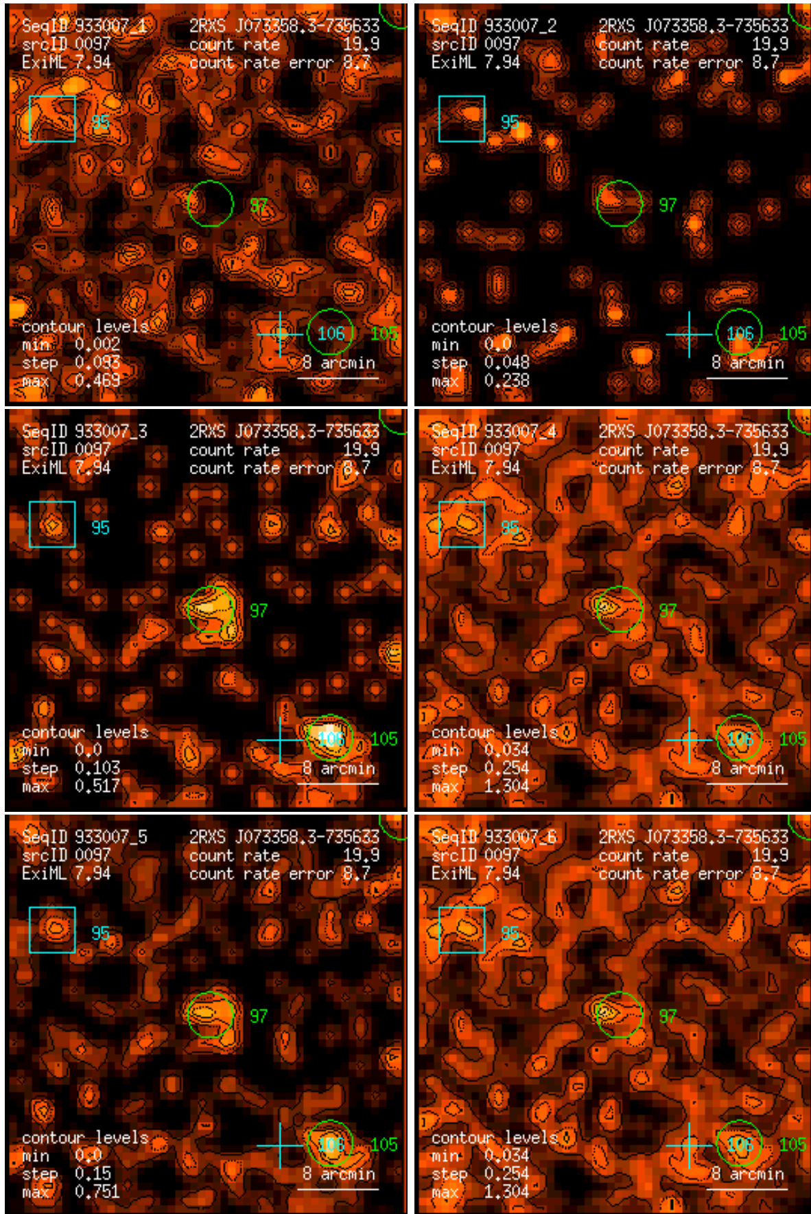
Figure 97: RASS 933007: detection 0097: band rate images, Gaussian filter: (1) PSPC channels 11 – 41, (2) 52 – 90, (3) 91 – 201, (4) 11 – 235, (5) 52 – 201, (6) 11 – 201. Broad band rates in counts/ks. Band rate contour levels in counts/ks/arcmin 2 .
