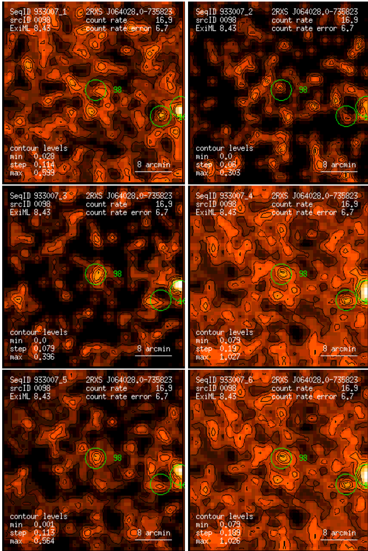
Figure 98: RASS 933007: detection 0098: band rate images, Gaussian filter: (1) PSPC channels 11 – 41, (2) 52 – 90, (3) 91 – 201, (4) 11 – 235, (5) 52 – 201, (6) 11 – 201. Broad band rates in counts/ks. Band rate contour levels in counts/ks/arcmin 2 .
