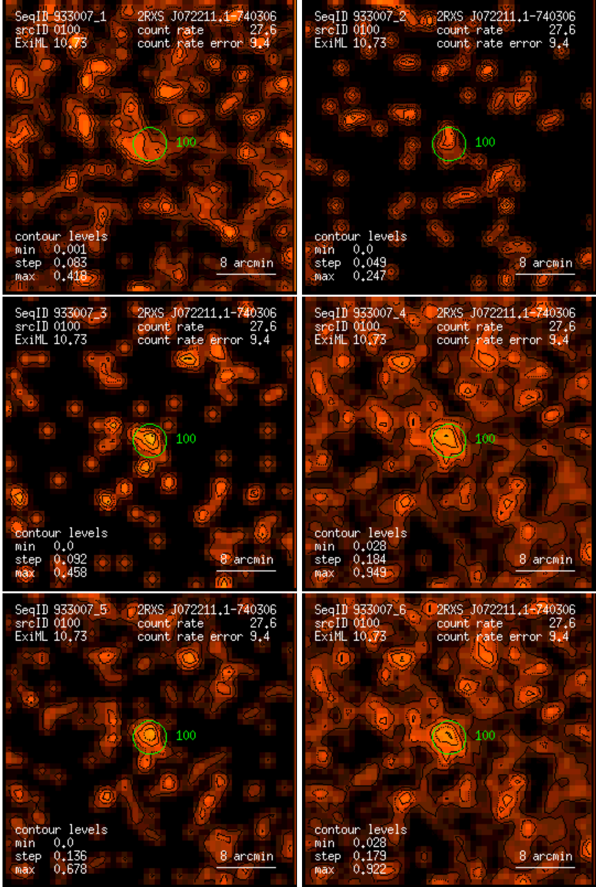
Figure 100: RASS 933007: detection 0100: band rate images, Gaussian filter: (1) PSPC channels 11 – 41, (2) 52 – 90, (3) 91 – 201, (4) 11 – 235, (5) 52 – 201, (6) 11 – 201. Broad band rates in counts/ks. Band rate contour levels in counts/ks/arcmin 2 .
