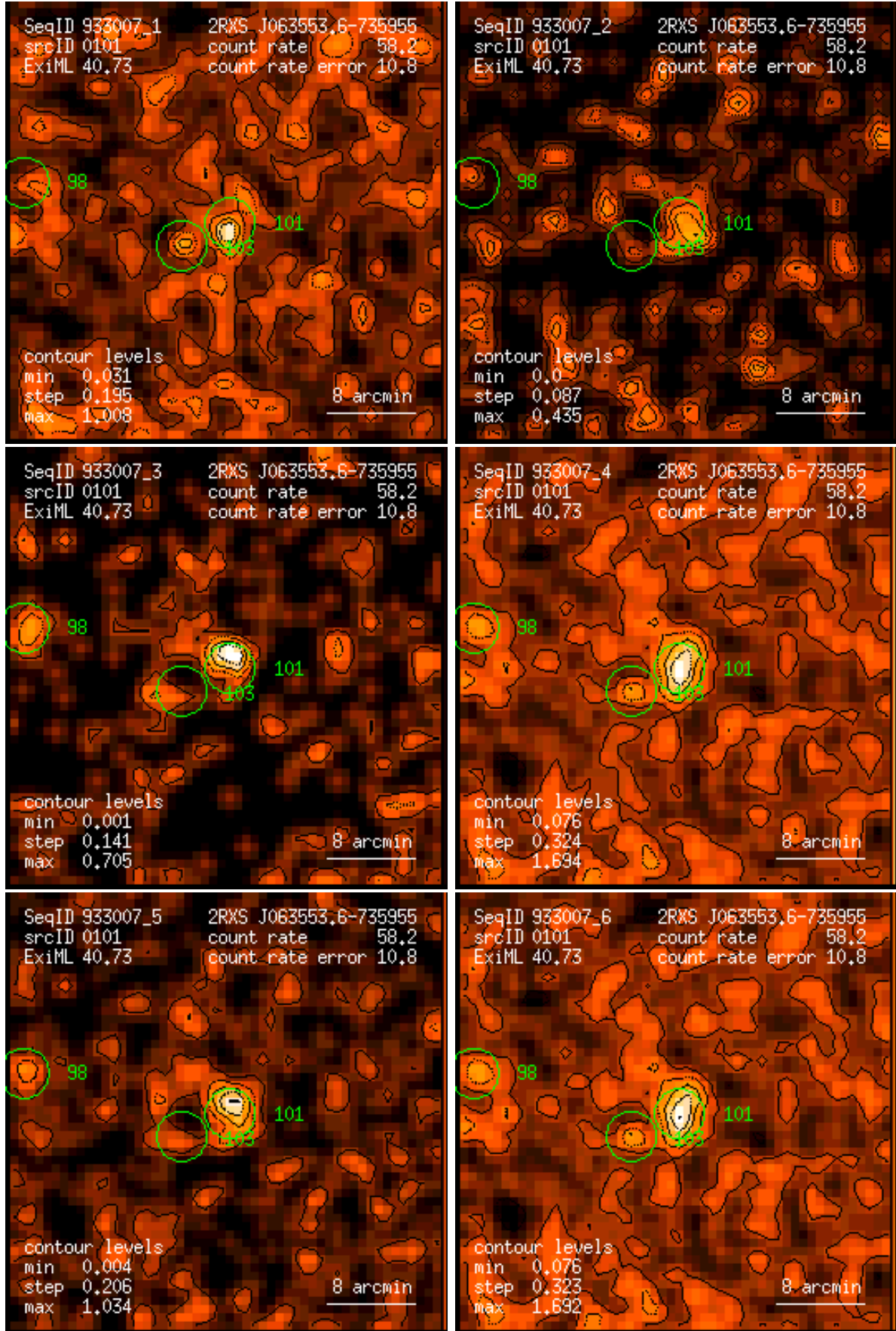
Figure 101: RASS 933007: detection 0101: band rate images, Gaussian filter: (1) PSPC channels 11 – 41, (2) 52 – 90, (3) 91 – 201, (4) 11 – 235, (5) 52 – 201, (6) 11 – 201. Broad band rates in counts/ks. Band rate contour levels in counts/ks/arcmin 2 .
