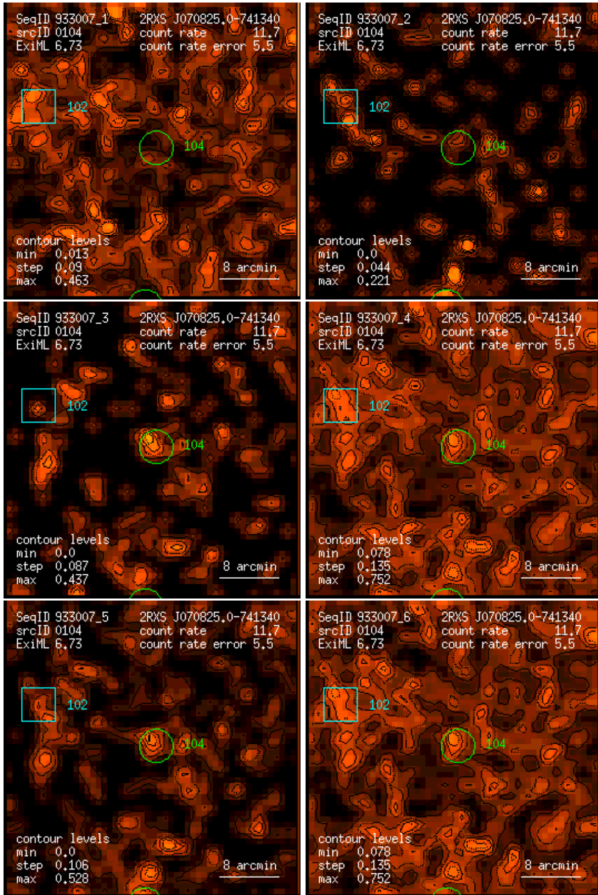
Figure 104: RASS 933007: detection 0104: band rate images, Gaussian filter: (1) PSPC channels 11 – 41, (2) 52 – 90, (3) 91 – 201, (4) 11 – 235, (5) 52 – 201, (6) 11 – 201. Broad band rates in counts/ks. Band rate contour levels in counts/ks/arcmin 2 .
