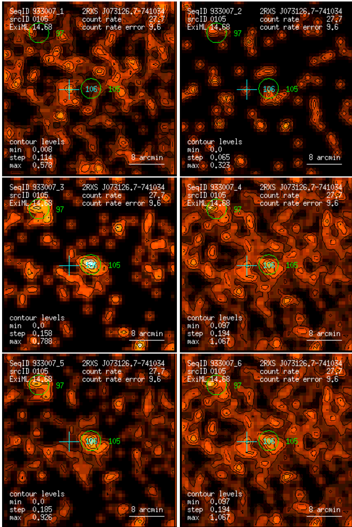
Figure 105: RASS 933007: detection 0105: band rate images, Gaussian filter: (1) PSPC channels 11 – 41, (2) 52 – 90, (3) 91 – 201, (4) 11 – 235, (5) 52 – 201, (6) 11 – 201. Broad band rates in counts/ks. Band rate contour levels in counts/ks/arcmin 2 .
