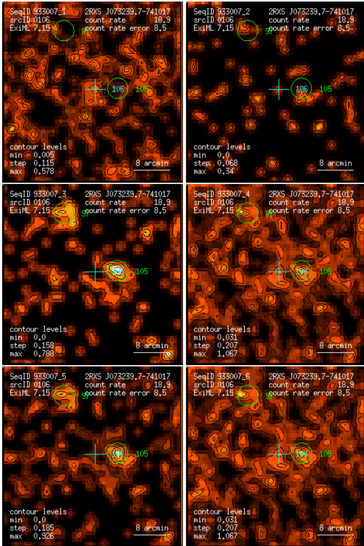
Figure 106: RASS 933007: detection 0106: band rate images, Gaussian filter: (1) PSPC channels 11 – 41, (2) 52 – 90, (3) 91 – 201, (4) 11 – 235, (5) 52 – 201, (6) 11 – 201. Broad band rates in counts/ks. Band rate contour levels in counts/ks/arcmin 2 .
