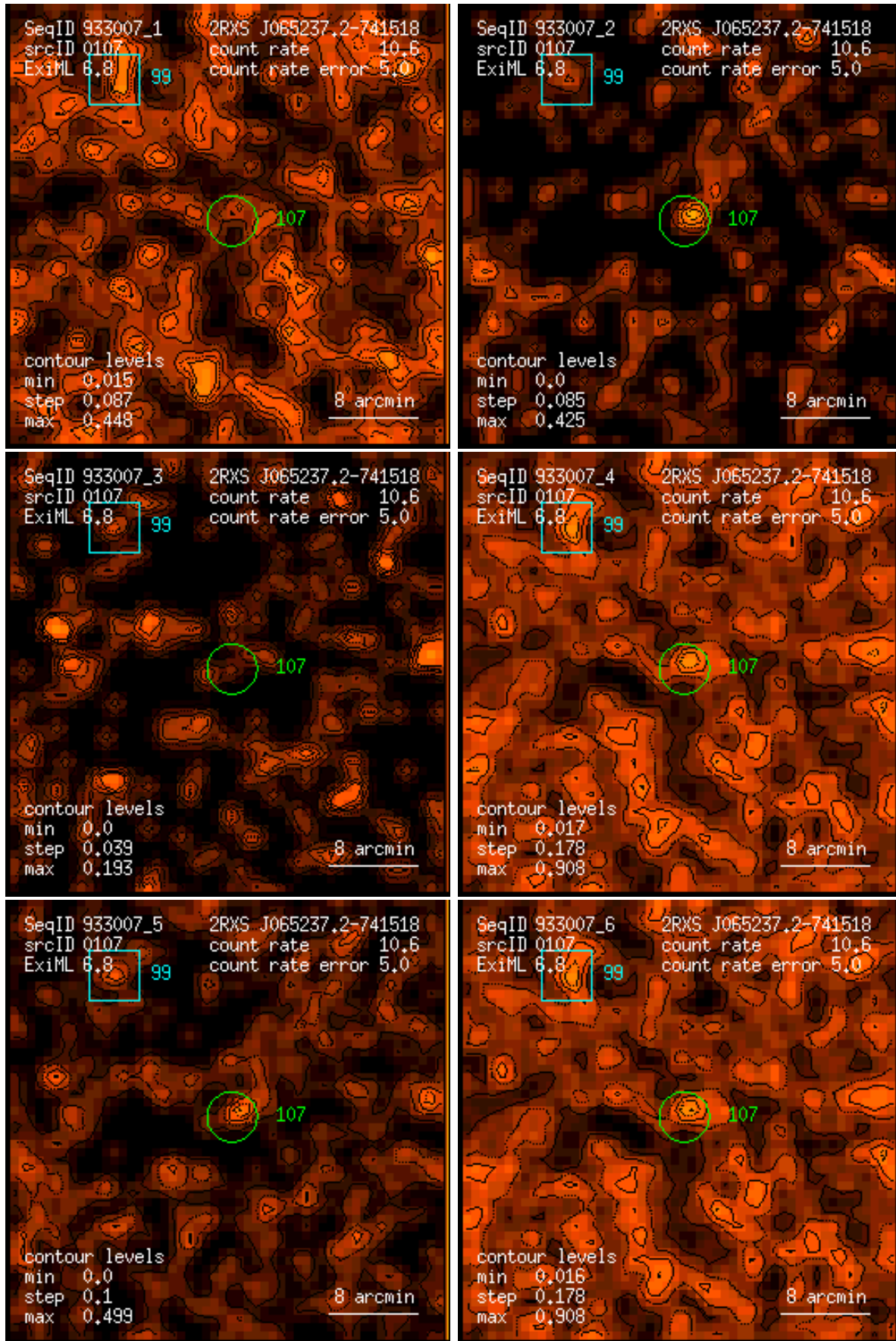
Figure 107: RASS 933007: detection 0107: band rate images, Gaussian filter: (1) PSPC channels 11 – 41, (2) 52 – 90, (3) 91 – 201, (4) 11 – 235, (5) 52 – 201, (6) 11 – 201. Broad band rates in counts/ks. Band rate contour levels in counts/ks/arcmin 2 .
