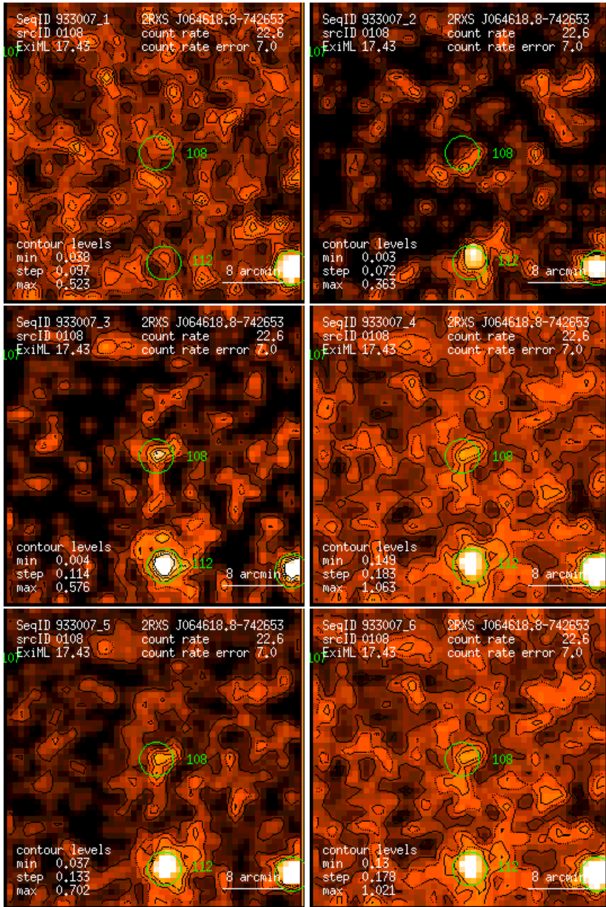
Figure 108: RASS 933007: detection 0108: band rate images, Gaussian filter: (1) PSPC channels 11 – 41, (2) 52 – 90, (3) 91 – 201, (4) 11 – 235, (5) 52 – 201, (6) 11 – 201. Broad band rates in counts/ks. Band rate contour levels in counts/ks/arcmin 2 .
