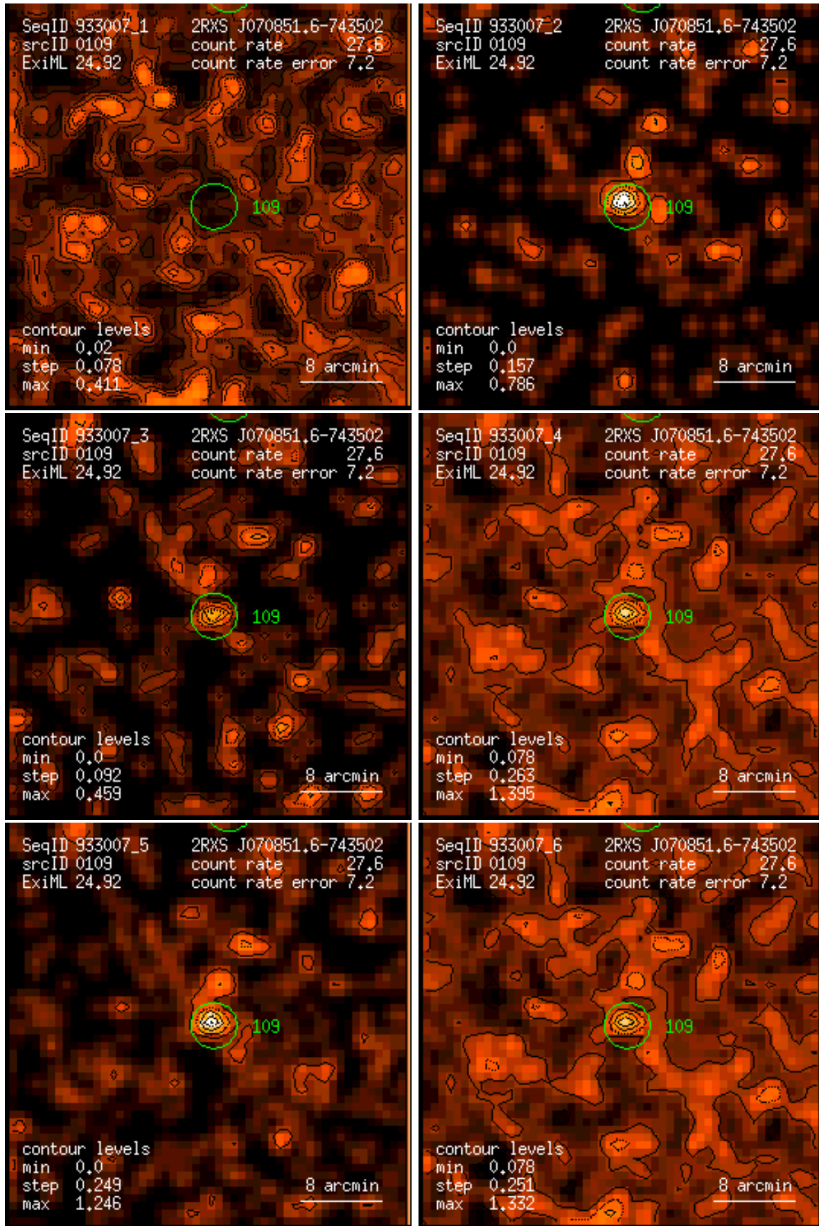
Figure 109: RASS 933007: detection 0109: band rate images, Gaussian filter: (1) PSPC channels 11 – 41, (2) 52 – 90, (3) 91 – 201, (4) 11 – 235, (5) 52 – 201, (6) 11 – 201. Broad band rates in counts/ks. Band rate contour levels in counts/ks/arcmin 2 .
