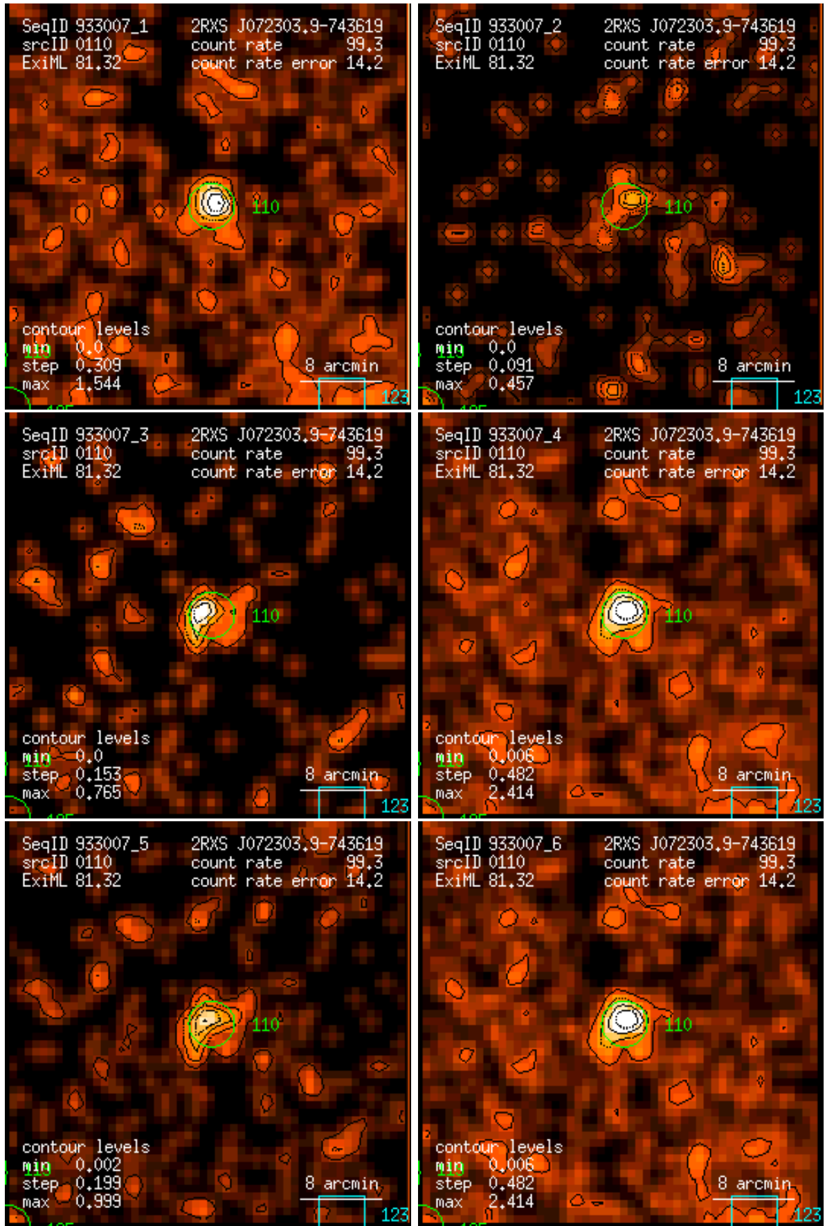
Figure 110: RASS 933007: detection 0110: band rate images, Gaussian filter: (1) PSPC channels 11 – 41, (2) 52 – 90, (3) 91 – 201, (4) 11 – 235, (5) 52 – 201, (6) 11 – 201. Broad band rates in counts/ks. Band rate contour levels in counts/ks/arcmin 2 .
