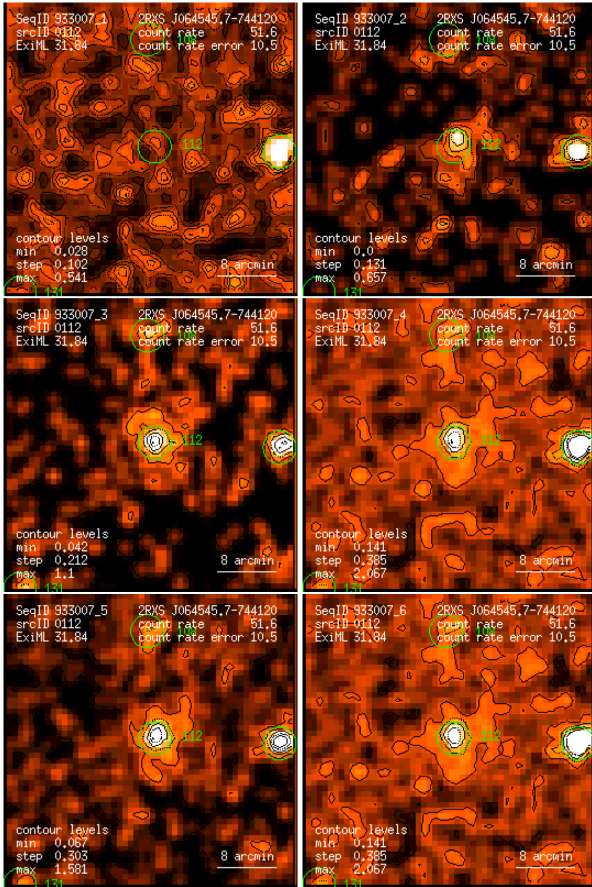
Figure 112: RASS 933007: detection 0112: band rate images, Gaussian filter: (1) PSPC channels 11 – 41, (2) 52 – 90, (3) 91 – 201, (4) 11 – 235, (5) 52 – 201, (6) 11 – 201. Broad band rates in counts/ks. Band rate contour levels in counts/ks/arcmin 2 .
