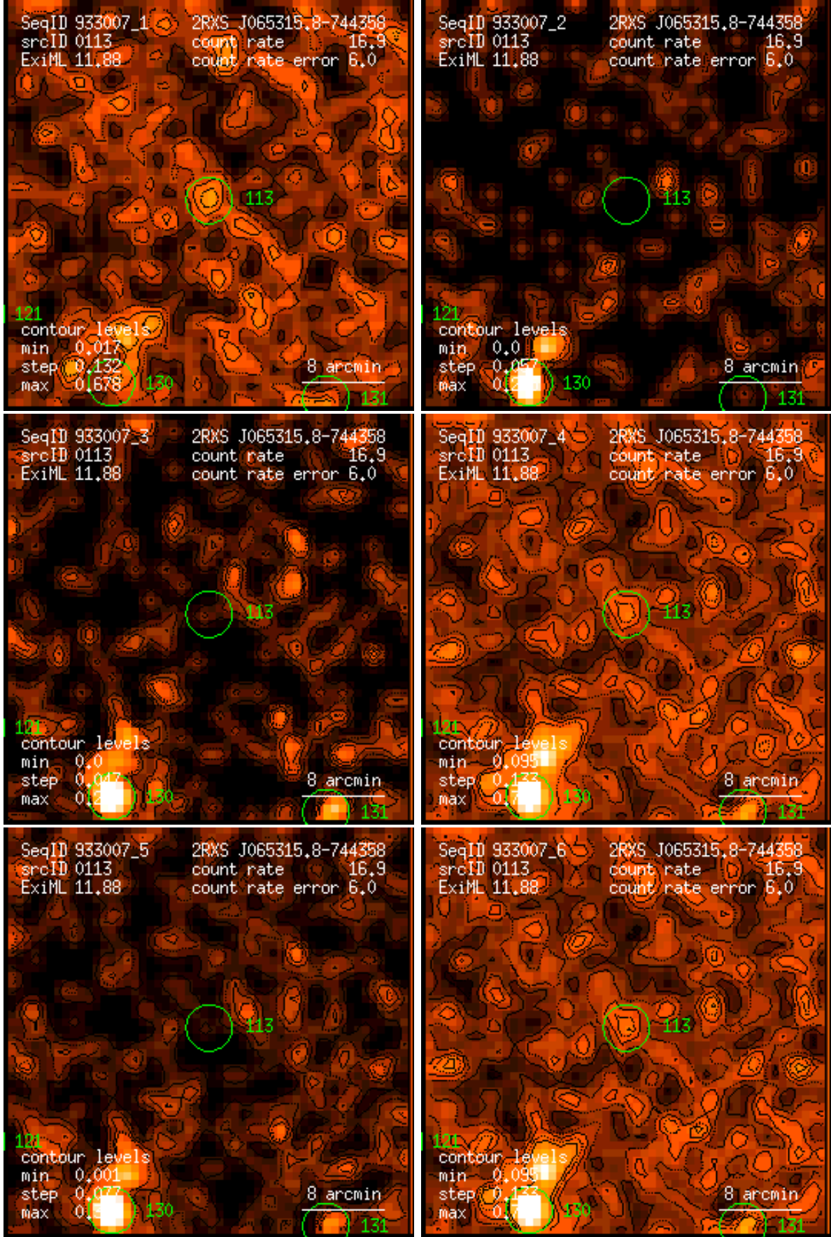
Figure 113: RASS 933007: detection 0113: band rate images, Gaussian filter: (1) PSPC channels 11 – 41, (2) 52 – 90, (3) 91 – 201, (4) 11 – 235, (5) 52 – 201, (6) 11 – 201. Broad band rates in counts/ks. Band rate contour levels in counts/ks/arcmin 2 .
