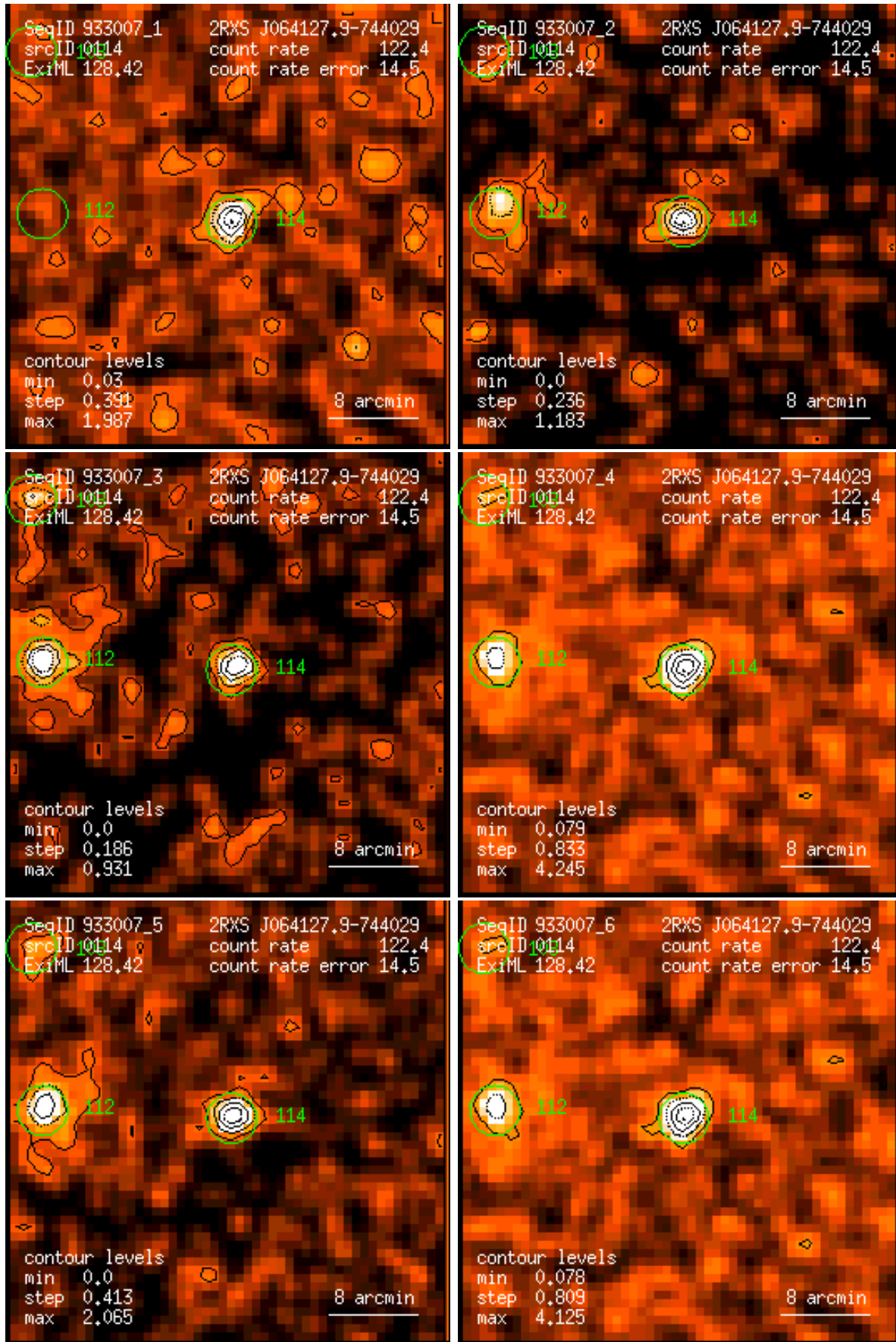
Figure 114: RASS 933007: detection 0114: band rate images, Gaussian filter: (1) PSPC channels 11 – 41, (2) 52 – 90, (3) 91 – 201, (4) 11 – 235, (5) 52 – 201, (6) 11 – 201. Broad band rates in counts/ks. Band rate contour levels in counts/ks/arcmin 2 .
