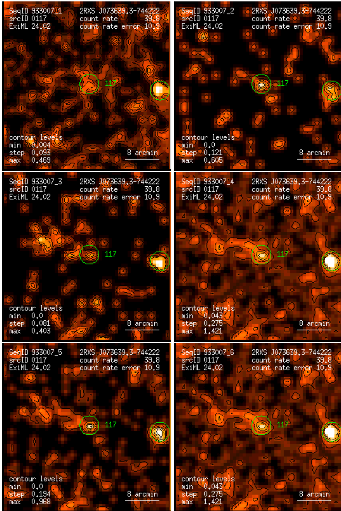
Figure 117: RASS 933007: detection 0117: band rate images, Gaussian filter: (1) PSPC channels 11 – 41, (2) 52 – 90, (3) 91 – 201, (4) 11 – 235, (5) 52 – 201, (6) 11 – 201. Broad band rates in counts/ks. Band rate contour levels in counts/ks/arcmin 2 .
